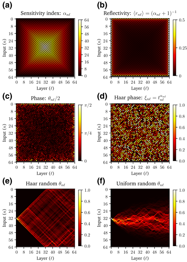
FIG. 2. (a) The sensitivity index \alpha_{n\ell} for N = 64 . (b) Checkerboard plot for the average reflectivity \langle r_{n\ell} \rangle in a rectangular mesh. (c) Decomposition of Ref. [10] for a Haar-random matrix yields phases close to cross state in the middle of the mesh. (d) The Haar phase \xi_{n\ell} for the rectangular mesh better displays the randomness. (e),(f) Field measurements (absolute value) from propagation at input 32 in (e) Haar and (f) uniform random initialized rectangular meshes with N = 64 .
