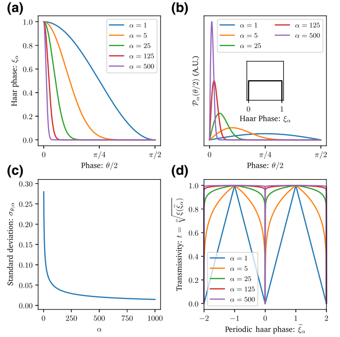
FIG. 3. (a) Plot of the relationship between \xi_{\alpha} and \theta . (b) We show that phase-shift standard deviation \sigma_{\theta;\alpha} decreases as \alpha increases. (c) A plot of \sigma_{\theta;\alpha} as \alpha increases. (d) The transmissivity of a MZI component as a function of a periodic Haar phase has a power-law relationship. The periodic Haar phase \tilde{\xi}_{\alpha} is mapped to the Haar phase by a function \xi : \mathbb{R} \rightarrow [0, 1] as discussed in Appendix G.
