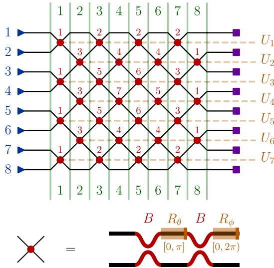
FIG. 1. Mesh diagram representing the locally interacting rectangular mesh for N = 8 . The inputs (and single-mode phase shifts at the inputs) are represented by blue triangles. Outputs are represented by purple squares. The MZI nodes are represented by red dots labeled with sensitivity index \alpha_{n\ell} (e.g., \alpha_{44} = 7 is the most sensitive node). The nodes represent the Givens rotation U_n (in orange) at vertical layer \ell (in green). Each photonic MZI node can be represented with 50:50 beam splitters B (red) and phase shifters R_\theta, R_\phi (orange), with required ranges 0 \leq \theta \leq \pi and 0 \leq \phi < 2\pi .
