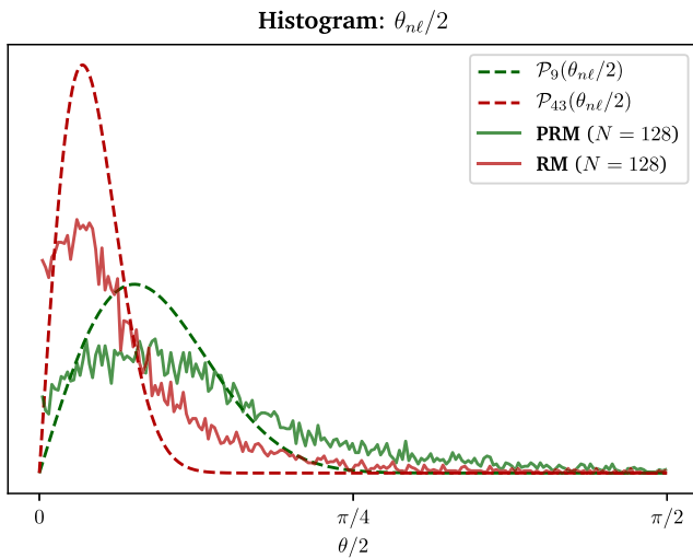
FIG. 13. Comparison of learned, normalized \theta_{n\ell} distributions for N = 128 rectangular (RM) and permuting rectangular (PRM) meshes with \mathcal{P}_\alpha(\theta/2) PDFs for \alpha = (N + 1)/3 = 43 (the average sensitivity index) and \alpha = \lfloor N/(2 \log N) \rfloor = 9 respectively. Note that permuting meshes have a larger tolerance, which eventually results in faster mesh optimization.
