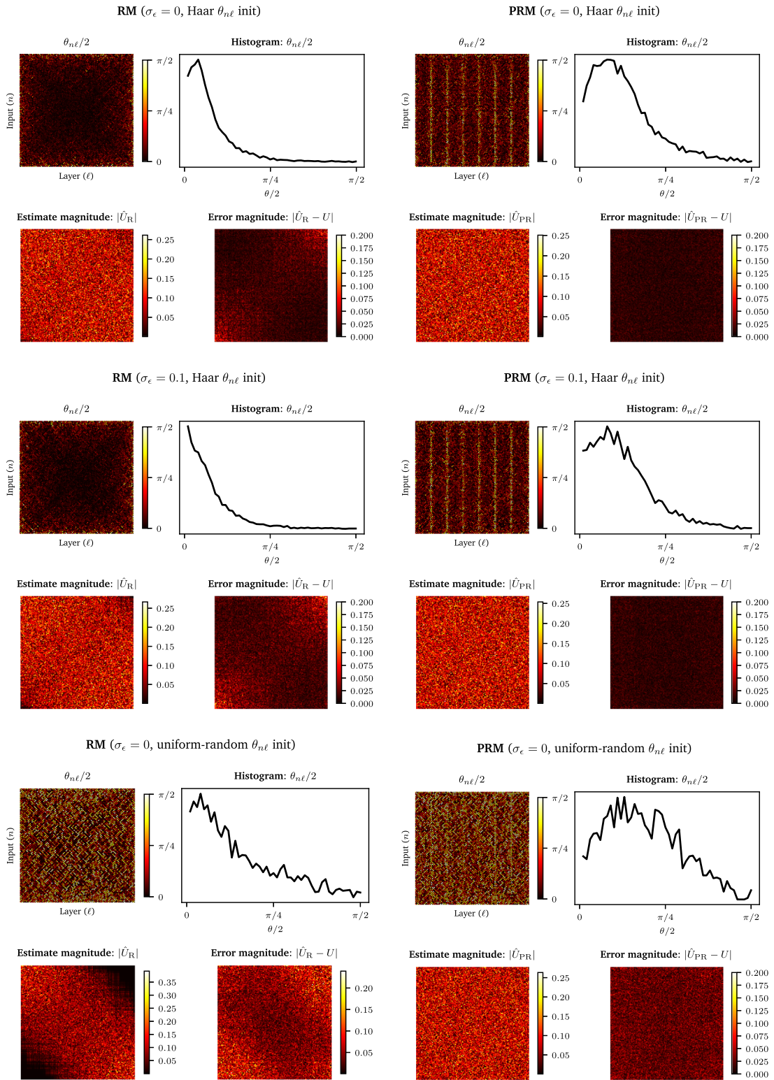
FIG. 12. Comparison of learned matrix errors and learned \theta_{n\ell} weights after 20,000 iterations for the Adam update at learning rate 0.0025 and batch size 256 for the simple unitary network. We consider two meshes: (1) rectangular mesh (RM) and (2) permuting rectangular mesh (PRM). We consider three conditions for each mesh: (1) ideal (with Haar random unitary initialization); (2) photonic beam-splitter error displacement \epsilon \sim \mathcal{N}(0, 0.01) ; (3) random initialization.
