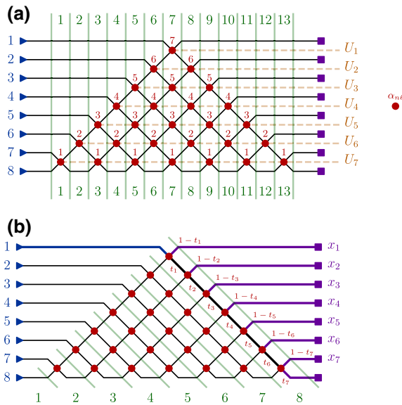
FIG. 8. Triangular mesh for N = 8 using (a) 2N - 3 vertical layers \ell , showing the sensitivity index \alpha_{n\ell} , and (b) N diagonal layers m , showing the transmissivity basis ( t_n in red) and the measurement basis ( x_n in purple).
