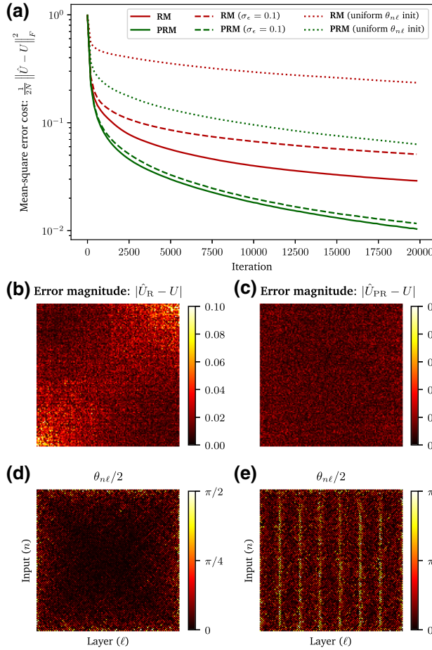
FIG. 6. We implement six different optimizations for N = 128 , where we vary the choice of permuting rectangular mesh (PRM) or rectangular mesh (RM); the initialization (random \theta_{n\ell} or Haar-initialized \theta_{n\ell} ); and photonic transmissivity error displacements [ \epsilon = 0 or \epsilon \sim \mathcal{N}(0, 0.01) , where \sigma_\epsilon^2 = 0.01 is the variance of the beam-splitter errors]. The conditions are 20,000 iterations, Adam update, learning rate of 0.0025, batch size of 256, simulated in tensorflow. (a) Comparison of optimization performance (defaults are Haar initialization and \epsilon_{n\ell} = 0 unless otherwise indicated). The optimized error magnitude spatial map for (b) rectangular mesh shows higher off-diagonal errors than (c) permuting rectangular. The optimized \theta_{n\ell} phase shifts (see Appendix G) for (d) rectangular meshes are close to zero (cross state) near the center as opposed to (e) permuting rectangular meshes, which have a striped pattern (likely due to initialization). Note that, by |\cdot| , we refer to the elementwise norm.
