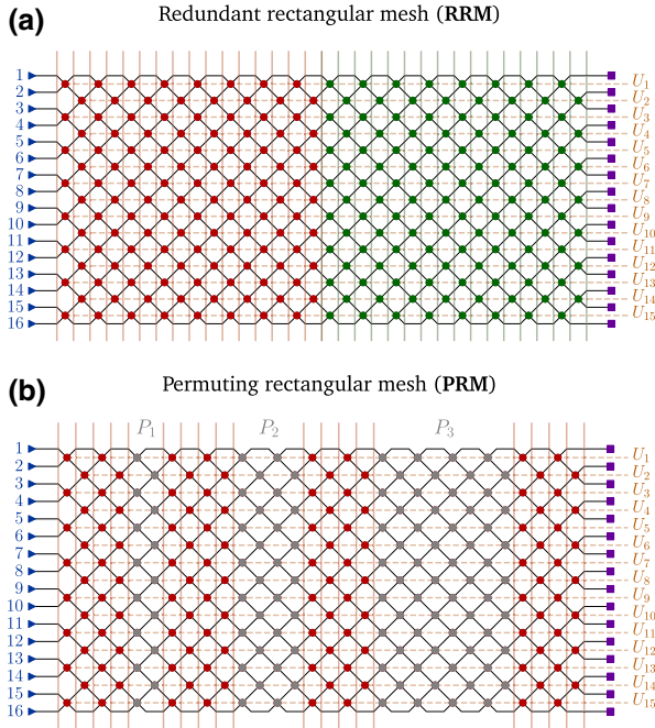
FIG. 4. (a) A 16 \times 16 rectangular mesh (red). Extra tunable layers (green) may be added to significantly reduce convergence time. (b) A 16-input, 30-layer permuting rectangular mesh. The rectangular permutation layer is implemented using either waveguide crossings or cross-state MZIs (gray).
