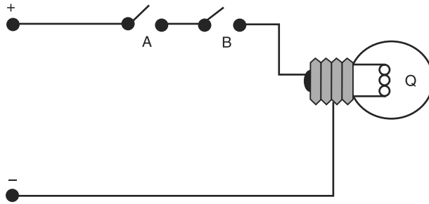
Circuit for AND gate
