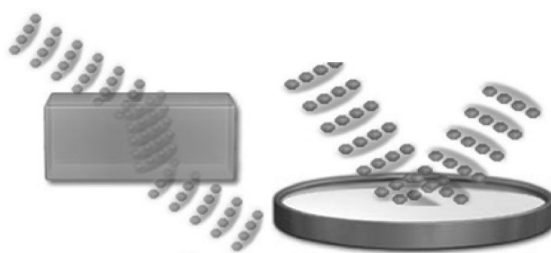
Fig.1.4. Behavior of light
