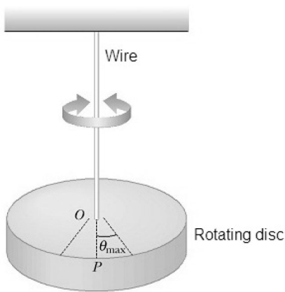
Fig.2-1; Torsional pendulum
