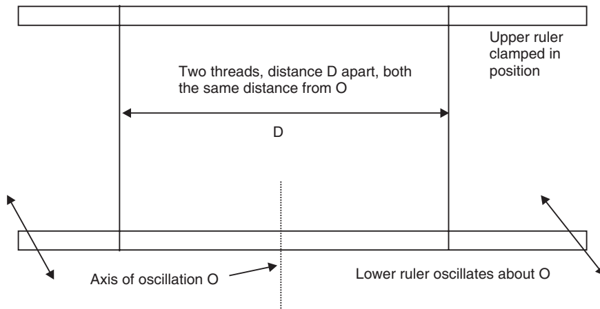
Fig.2-3; Bifilar suspension
