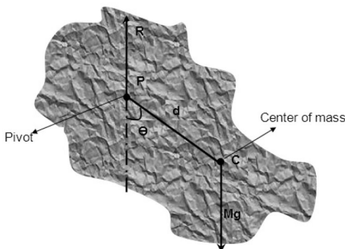
Fig.2-2; Compound pendulum
