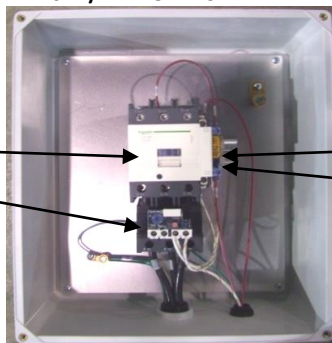
J1A/ HP PUMP STARTER
