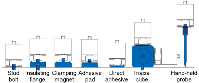
Figure 18: Mounting methods for accelerometers
