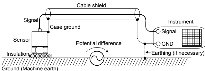
Figure 23: Insulated sensor mounting avoids ground loops
