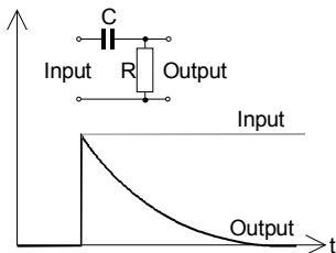
Figure 15: Step response of IEPE transducers
