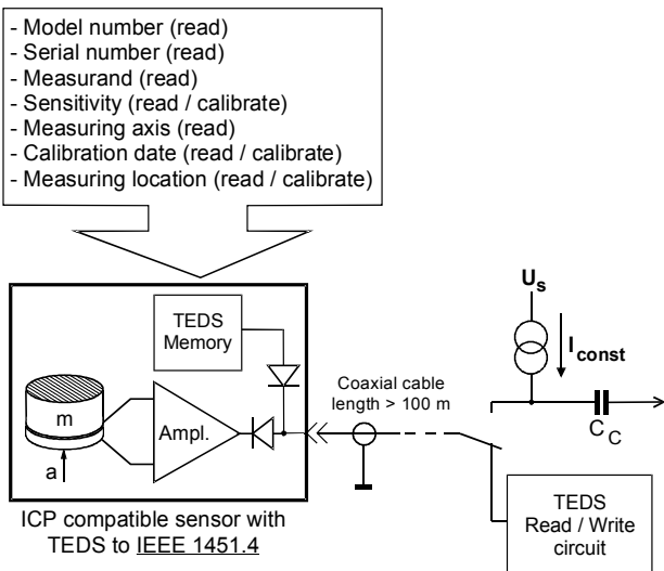
Figure 16: TEDS principle
