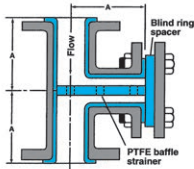
Strainer Tee
