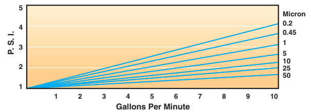
Initial pressure drop per 10" cartridge
