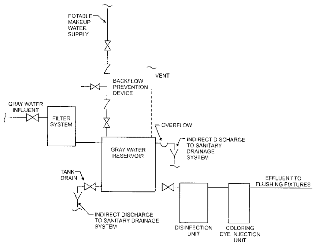
FIGURE 1301.1(2) GRAY WATER RECYCLING SYSTEM FOR FLUSHING WATER CLOSETS AND URINALS
