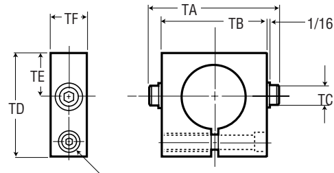
Trunnion
