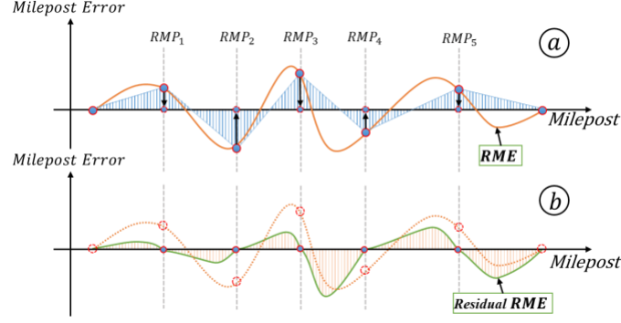
Fig.9 Illustration of the PS-Model process.
