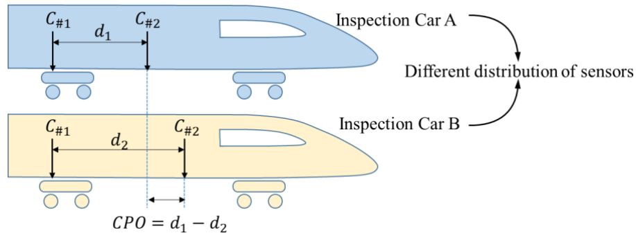
Fig.3: Sketch map of the CPO and track geometries. C_{\#1} and C_{\#2} represent two different types of track geometry; d_1 and d_2 are the relative distances between the measurement locations of C_{\#1} and C_{\#2} , for inspection Car A and Car B, respectively.
