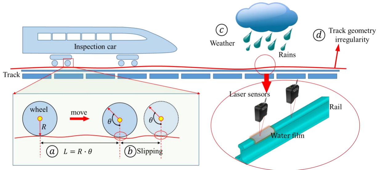
Fig.2: Positioning principle of the inspection car and the causes of the positional errors. (a) shows the mileage measuring principle; (b) shows the degraded adhesive conditions that leads to relative slippage between rail and wheel; (c) shows unforeseen influences such as weather; (d) track geometry irregularity.
