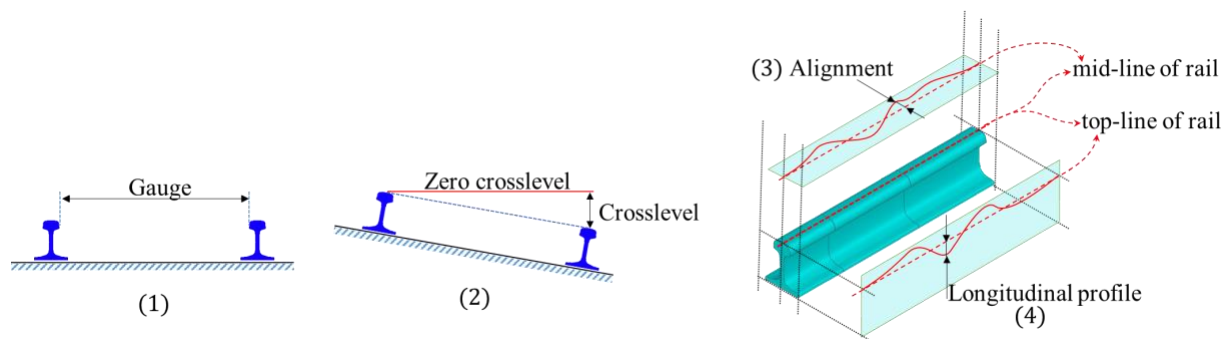
Fig.1: Schematic diagrams of track gauge, crosslevel, alignment and longitudinal profile
