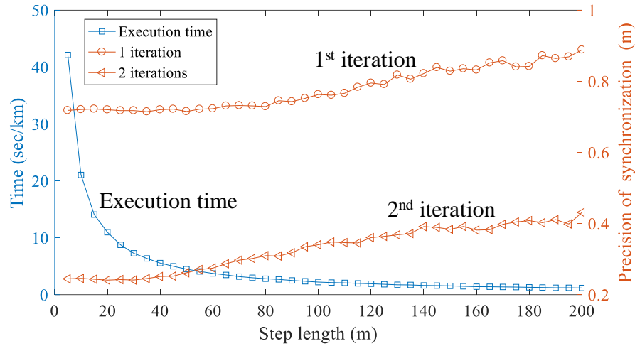
Fig.16 The execution time and precision P_r(p = 99.7\%) of position synchronization considering different matching step ds .
