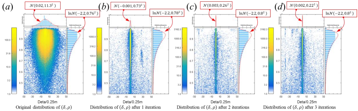
Fig.14 The joint distribution of value pairs (\delta, \rho) . (a), (b), (c) and (d) show the distributions of the original data, and the data after one, two and three iterations respectively.
