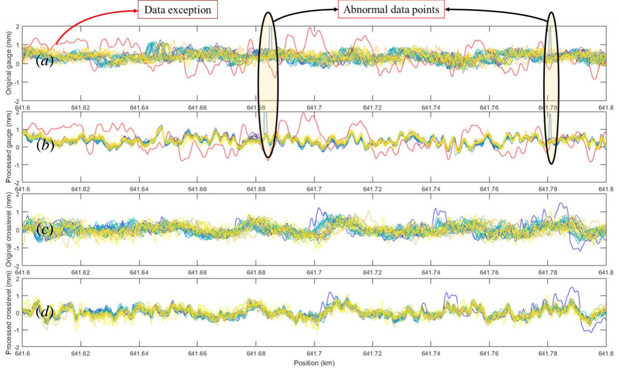
Fig.13 Comparison of the waveform before and after position synchronization (Channel #1 gauge). (a) and (b) illustrate the waveforms of the original and processed gauge, respectively; (c) and (d) illustrate the waveforms of the original and processed crosslevel, respectively.
