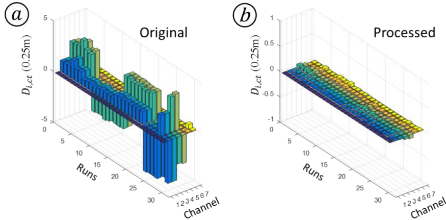
Fig.12 The estimation of CPO; (a) shows the CPO of original data; (b) illustrates the CPO of the processed data.
