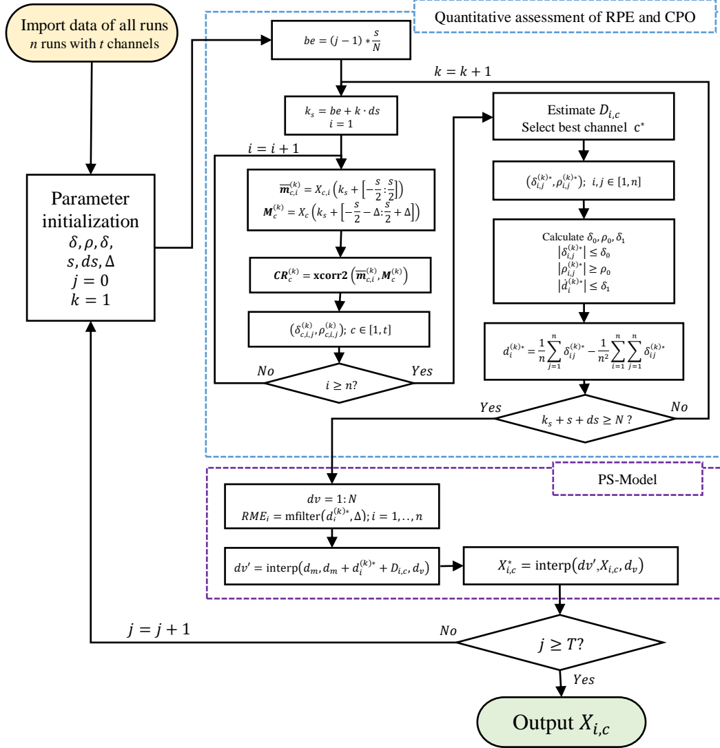
Fig.17 The OI-Algorithm flow chart.
