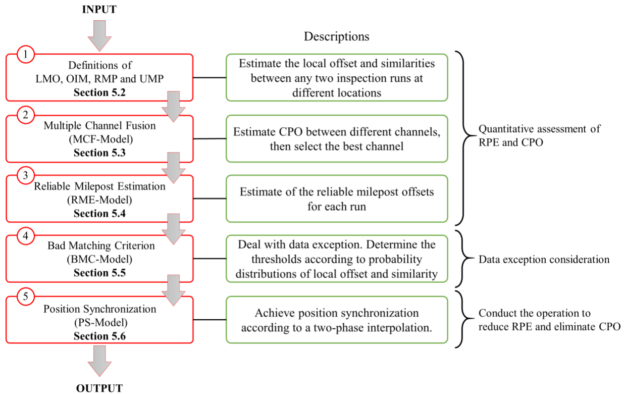
Fig.5: Overall model framework.
