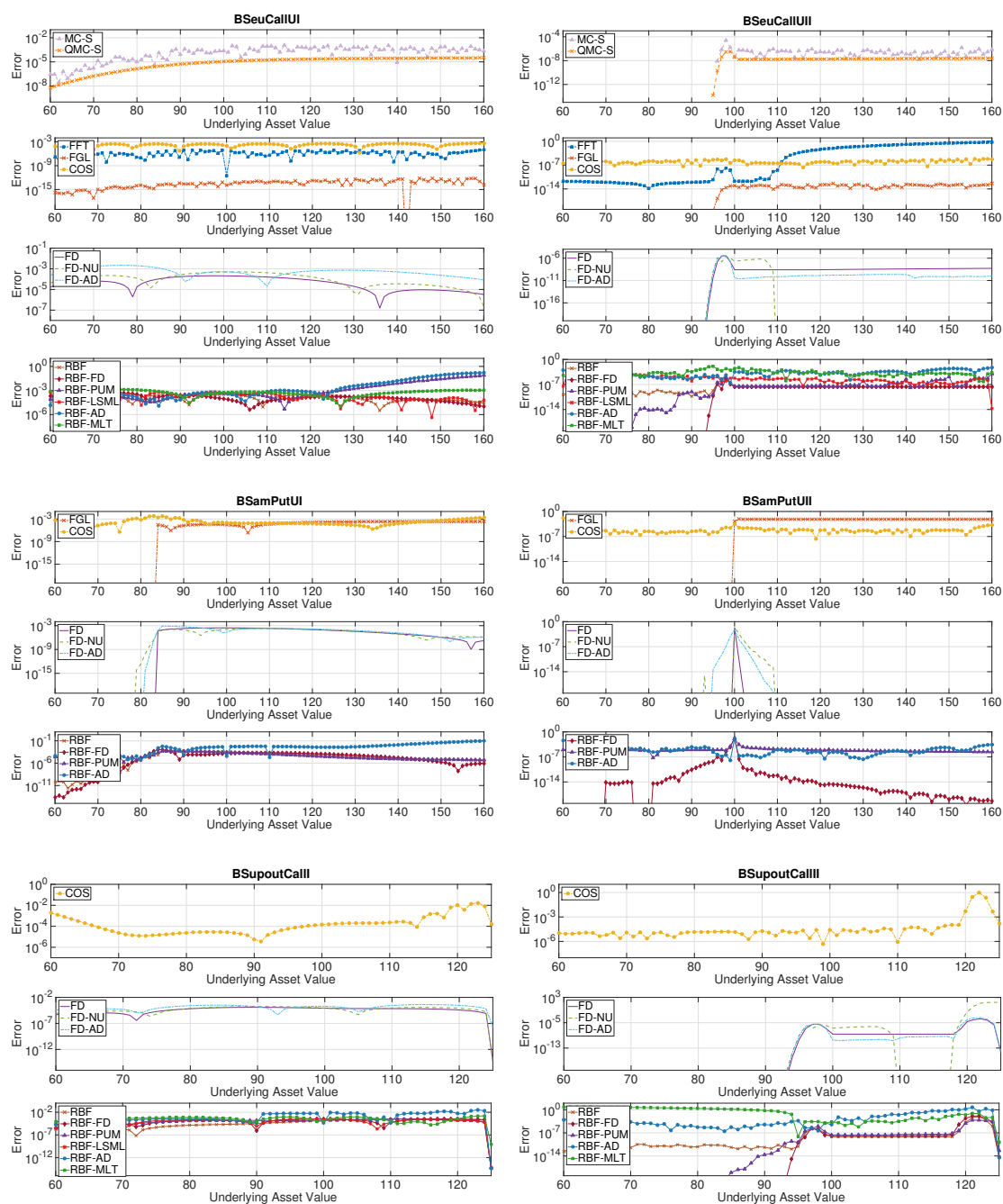
Figure 1. Problem 1a) European call option (top group), 1b) American put option (middle group), and 1c) Up-and-out call option (bottom group). For each problem, results for standard parameters to the left, and for challenging parameters to the right. Absolute error in the solution u for t = 0 and 60 \leq s \leq 160 when the relative error in u is less than 10^{-4} at t = 0 and s = 90, 100, 110 for standard parameters and s = 97, 98, 99 for challenging parameters. For the barrier option, results are shown up to the barrier at s = 125 .
