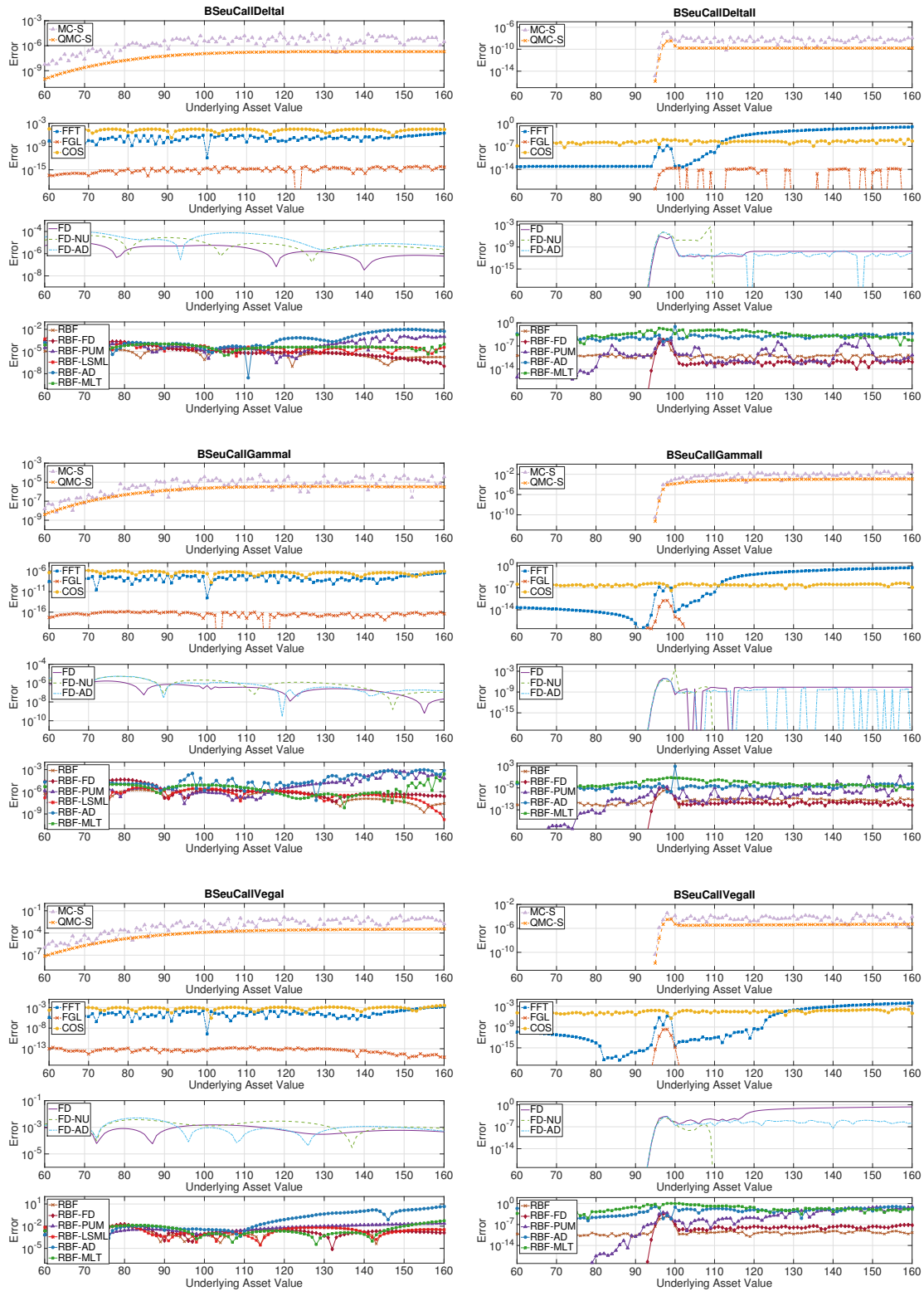
Figure 2. Problem 1a) European call option. Errors in the hedging parameters \Delta (top group), \Gamma (middle group), and \mathcal{V} (bottom group). For each problem, results for standard parameters are shown to the left, and for challenging parameters to the right. Absolute errors in the hedging parameters for t = 0 and 60 \leq s \leq 160 when the relative error is less than 10^{-4} at t = 0 and s = 90, 100, 110 for standard parameters and s = 97, 98, 99 for challenging parameters.
