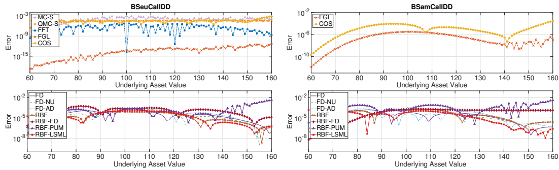
Figure 3. Problem 2 a) European call with dividends (left) and 2b) American call with dividends (right). Error in the solution u for t = 0 and 60 \leq s \leq 160 when the relative error in u is less than 10^{-4} at t = 0 and s = 90, 100, 110 .
