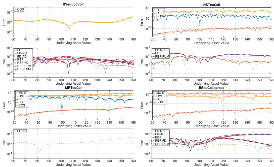
Figure 4. Problem 3 Local volatility, smooth function (top left), Problem 4 Heston (top right), Problem 5 Merton (bottom left), and Problem 6 Spread option (bottom right). Absolute error in the solution u for t = 0 and 60 \leq s \leq 160 when the relative error in u is less than 10^{-4} at t = 0 and s = 90, 100, 110 for Local volatility and Merton, and for Heston with variance v = 0.0225 . For the spread option, the error is measured in (s_1, s_2) = (100, 90), (100, 100), (100, 110), (90, 100), (110, 100) , and is plotted for 60 \leq s_1 \leq 160 , and s_2 = 100 .
