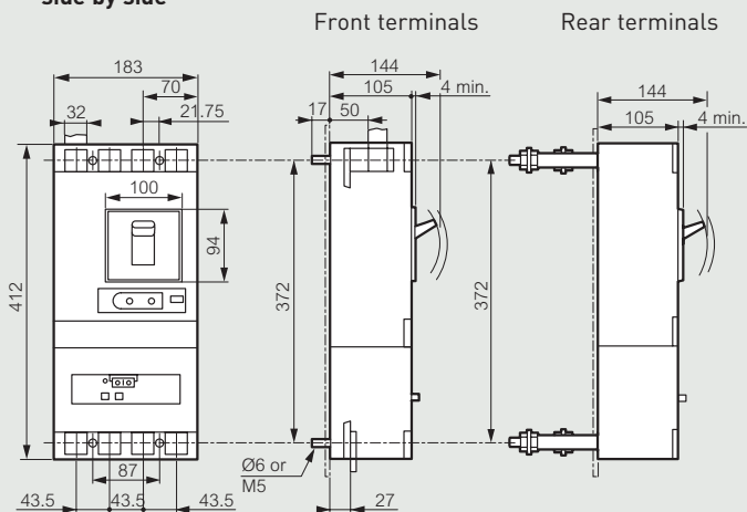
■ Fixed version with earth leakage module mounted side by side
