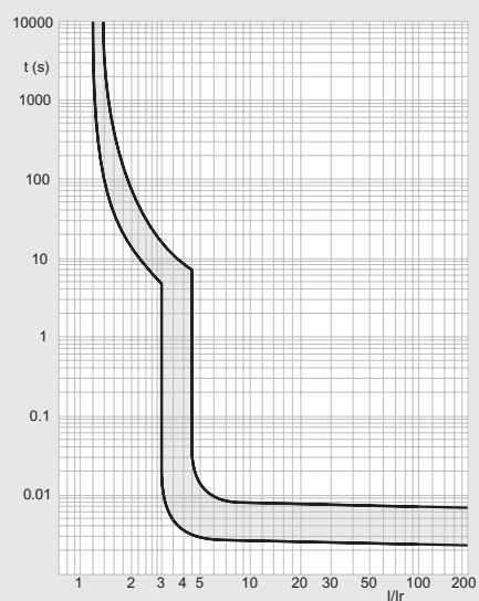
Curve B
