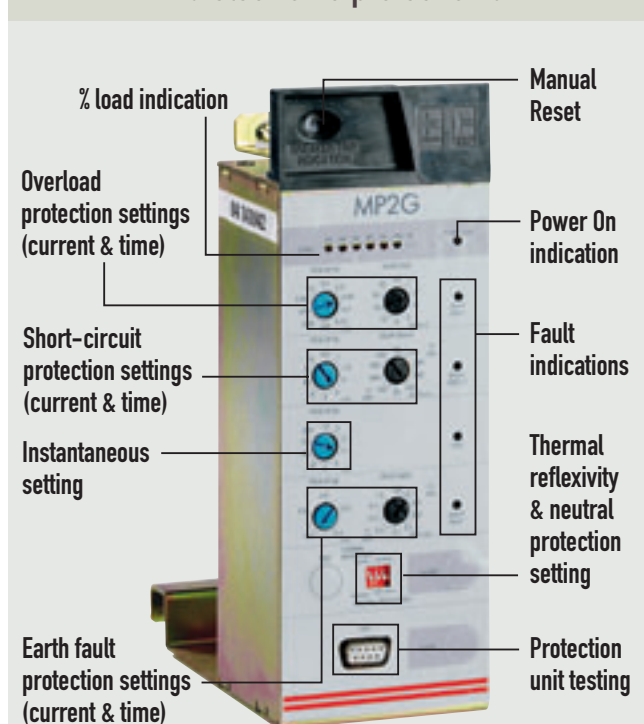
MP 2G electronic protection unit
