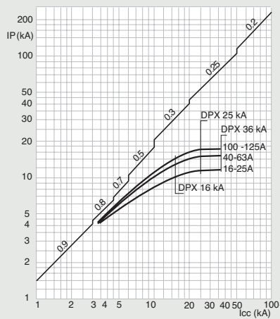
DPX 125
