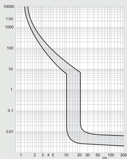
Curve D
