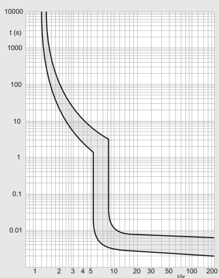
Curve C
