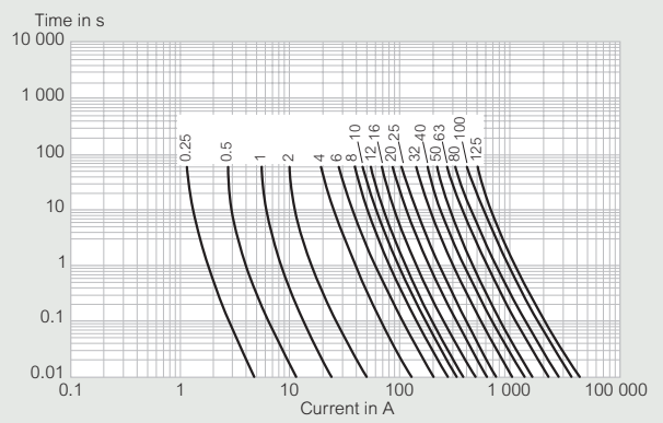
aM type
