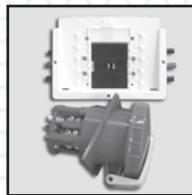
MPL1142XA Lighthouse® • Lighthouse SS • Admiral 100A 1ø Faceplate Assembly with Breakers and Plate (120/250V)
