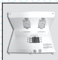
MPL1135A, MPL1135A-2 Newport Harbor Mate 30A-30A Faceplate Assembly with Breakers (Without Stand) 30A-30A Faceplate Assembly with Breakers (With Stand)
