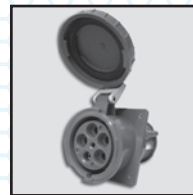
MPL5100R7W 100A 277/480V 5-Wire Pin and Sleeve (Red)
