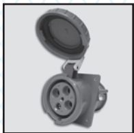
MPL4100R7W 100A 480V 4-Wire Pin and Sleeve (Red)
