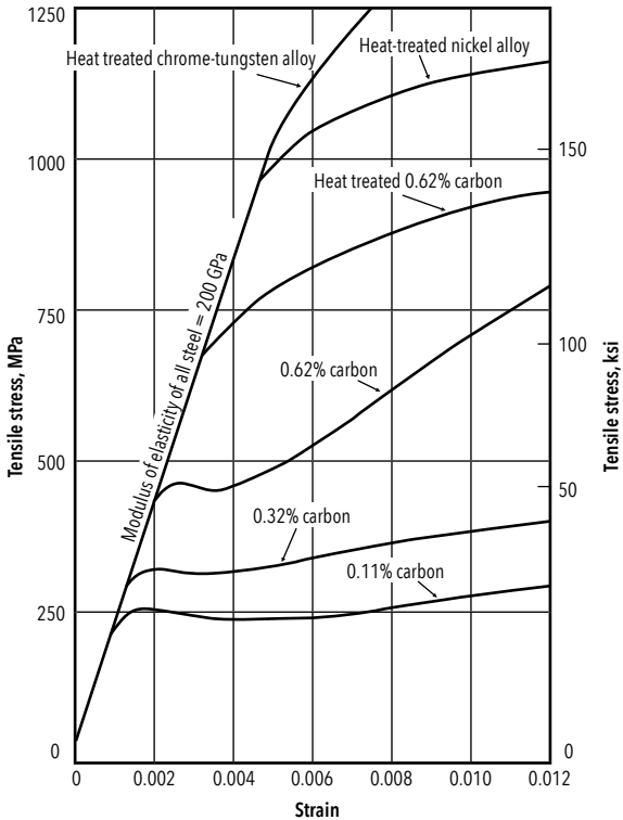
Atlas of Stress-Strain Curves, Second Edition; ASM International, 2002
