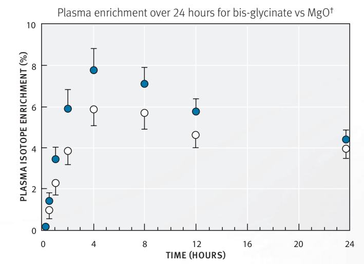
Plasma isotope enrichment vs time for the first 24 hours after Mg ingestion. Data for both Mg-labeled chelate (●) and Mg Oxide (○) are shown as the group average ± SEM for all time points. Study subjects with the greatest impairment in magnesium absorption showed substantially greater tolerance and absorption of magnesium when it was delivered in the bis-glycinate form.
