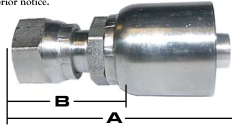
316 OFT (O-RING FACE SEAL)
