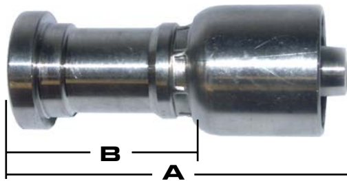
316 CODE 61 FLANGE
