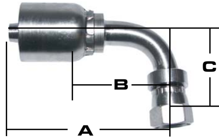
316 FEMALE JIC 90°
