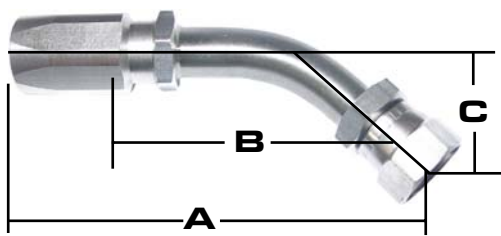
316 FEMALE JIC 45°
