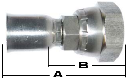
316 SWIVEL FEMALE BSP 60° CONE
