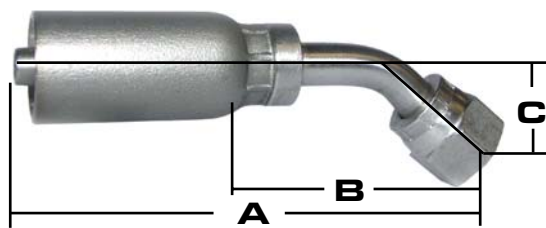
303 FEMALE JIC 45°
