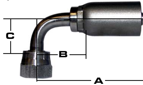
303 SWIVEL FEMALE BSP 60° CONE 90°
