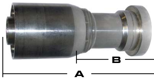
316 CODE 62 FLANGE
