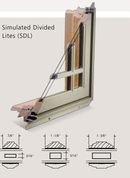
Full-Surround (FS) and KD Removable Wood Grilles (Available on direct set only)
