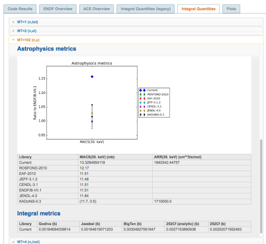
Figure 4. Screenshot of the new integral quantity report being phased into the ADVANCE QA reports. Metrics such as the 30 keV Maxwellian Averaged Cross Section (MACS) are compared to results from the KADONIS library [9] and a variety of other databases. Comparison data was taken from Ref. [10].
