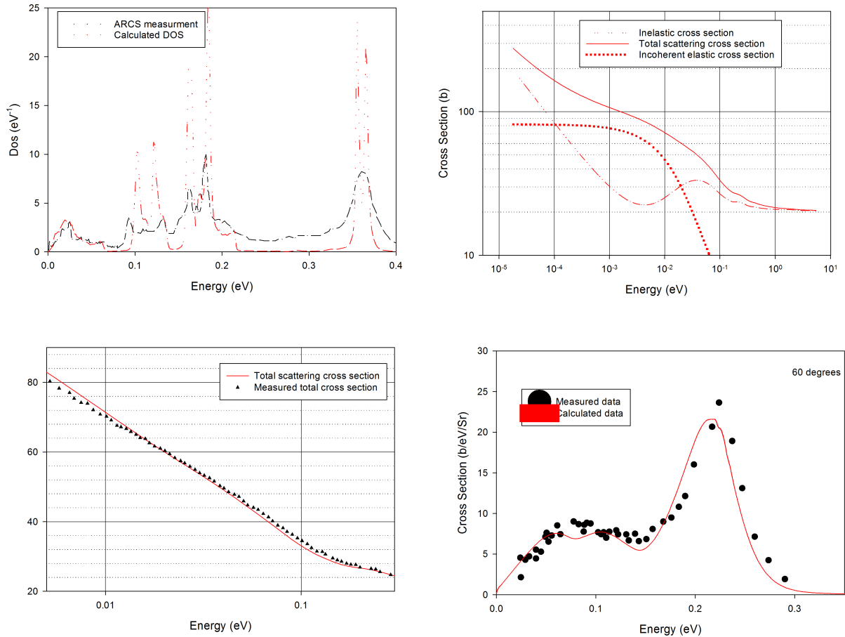
Figure 2. The polyethylene thermal scattering law evaluation from North Carolina State University in ENDF/B-VIII. In the upper left hand panel, we show the density of states used in the polyethylene evaluation along with the data from Lavelle, et al. [5]. In the upper right hand panel, we compare the total scattering, inelastic scattering and the incoherent elastic scattering cross sections. In the lower left panel, we show the total scattering cross section compared the data taken from EXFOR [4]. In the lower right panel, we show the incoherent elastic cross section compared to the data from EXFOR [4]. This figure taken from Ref. [6].
