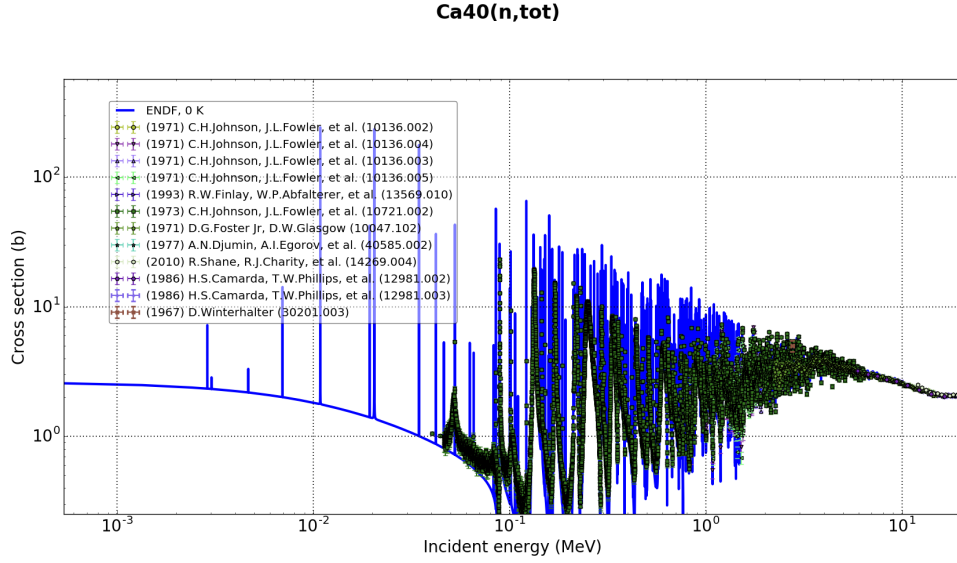
Figure 1. ^{40}\text{Ca}(n,\text{tot}) cross section from the new ORNL evaluation in ENDF/B-VIII. The new evaluation is given in blue and the world's collection of total reaction data as stored in EXFOR [4] are shown in the symbols.
