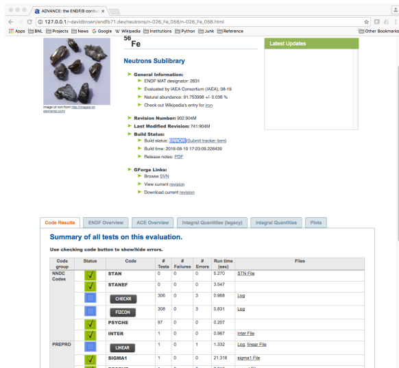
Figure 3. Screenshot of a typical ADVANCE build report. Successful builds are denoted with the green checkmark, builds with errors are given the blue box and failed builds are given a red “bomb”. Fortunately there are no failures in this build. Error messages can be reviewed using the black button for each build.
