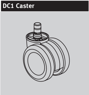
DC1 Caster 2 1/2-inch-diameter double-wheel braking caster; black nylon wheels and yoke; quiet roll technology Applicable on: New Aeron Chairs
