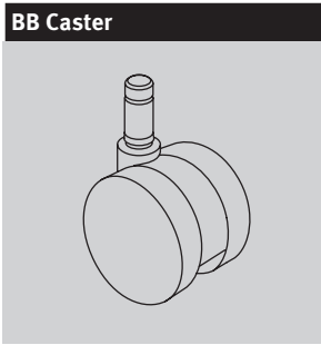
BB Caster 2 1/2-inch-diameter hard double-wheel caster; black nylon wheels and yoke; for use on carpet only Applicable on: New Aeron® Chairs Caper® Chairs Embody® Chairs Equa 2® Chairs Ergon 3® Chairs Lino™ Chairs Mirra® 2 Chairs Sayl Chairs Verus™ Chairs
