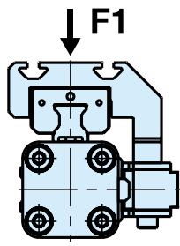
Loading 1 Top carrier
