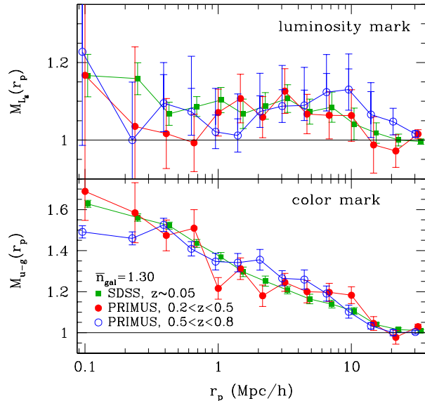
FIG. 19.— Luminosity (upper panel) and color (lower panel) mark correlation functions for low and high-redshift PRIMUS samples ( z < 0.5 and z > 0.5 , solid and open circles), with the number density \bar{n}_{\text{gal}} = 1.30 \cdot 10^{-2} h^3 \text{Mpc}^{-3} (see Table 9). The extended upper errors of the high- z luminosity mark indicate the upper error bars when the COSMOS field is included. SDSS results (green squares) are also shown, for comparison, and the points are slightly offset in \log(r_p) , for clarity. There appears to be no evolution of the luminosity- and color-environment correlations between z \sim 0 and z \sim 1 .
