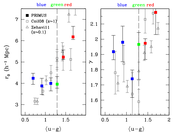
FIG. 15.— Clustering length ( r_0 , left) and slope ( \gamma , right) as a function of u-g color. For comparison, we show the results of Coil et al. (2008; open square points) and Zehavi et al. (2011; open triangles).
