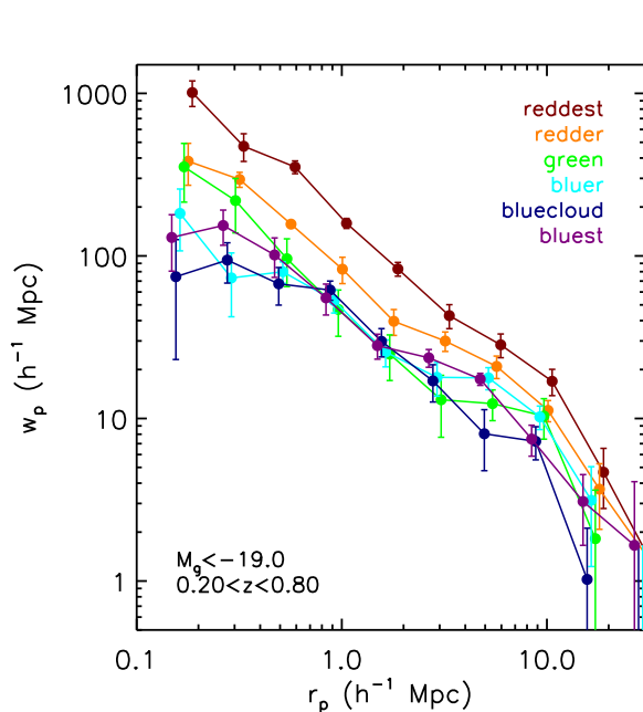
FIG. 14.— Projected correlation functions for finer color bin samples (described in Table 4): two (three) bins for the red (blue) sequence, and an intermediate ‘green valley’ bin. The points are slightly offset in \log(r_p) , for clarity.
