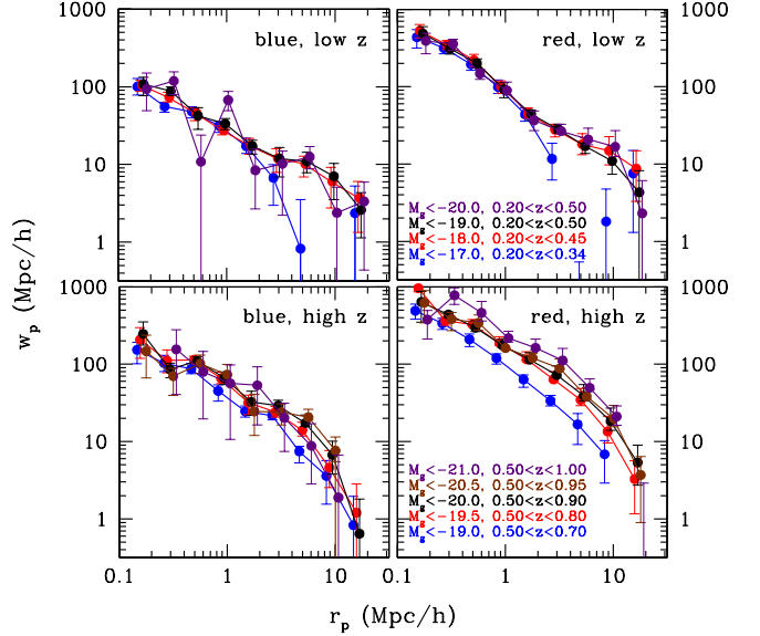
FIG. 10.— Projected correlation functions for blue and red galaxies (left and right panels), for L -threshold samples at low and high redshift (upper and lower panels).
