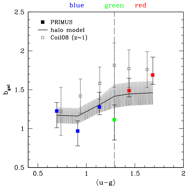
FIG. 16.— PRIMUS (filled points) color-dependent bias, for the finer color binned samples. For comparison, the results from the halo model-based mock catalog (black solid line) and Coil et al. (2008; open points) are shown. As before, the Coil et al. results are shifted to account for the different values of \sigma_8 ; but note that their results are at z \sim 1 , while ours have a mean redshift of \langle z \rangle \approx 0.5 .
