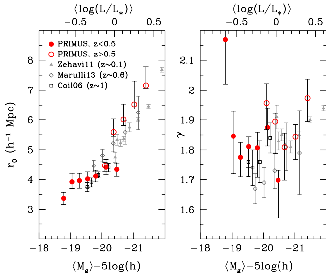
FIG. 7.— The clustering length ( r_0 ) and slope ( \gamma ) for all the luminosity-threshold samples, estimated from power-law fits to the correlation functions. The lower x -axis shows the mean g -band magnitude, while the upper one shows the g -band luminosity relative to L_* of the luminosity function. The filled red circles are the PRIMUS samples with 0.20 < z < 0.50 and the open red circles are those with 0.5 < z < 1.0 . The 1\text{-}\sigma errors are estimated with the 16 and 84 percentiles of the jackknife subsamples. Note that the high- z r_0 results at L \gtrsim L_* are affected by the large structure in the COSMOS field, which is in all but one of the subsamples; consequently, COSMOS raises the upper error bar. For comparison, we show the results of Coil et al. (2006b; DEEP2 survey; square points), Marulli et al. (2013; VIPERS; diamonds), and Zehavi et al. (2011; SDSS; triangles).
