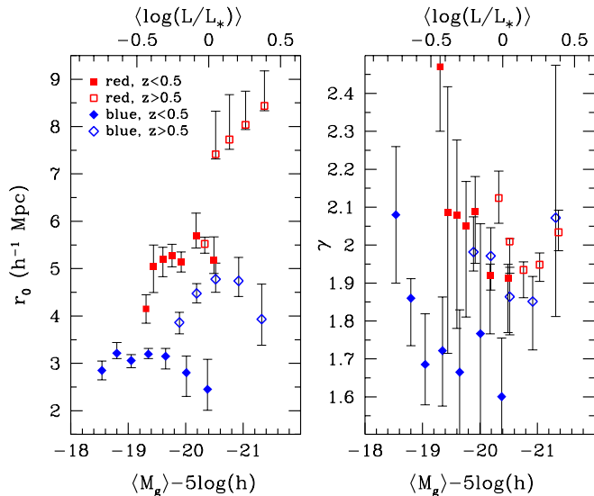
FIG. 12.— Clustering length ( r_0 , left) and slope ( \gamma , right) for red and blue galaxies (indicated by red square and blue diamond points), as a function of luminosity. Solid and open points are results at low and high redshift, respectively. The DEEP2 and SDSS results of Coil et al. (2008) and Zehavi et al. (2011; not shown) are similar, though the latter have slightly higher red galaxy r_0 at L \ll L_* .
