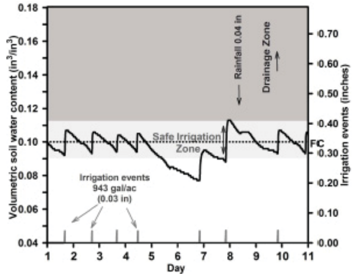
Figure 4. Example of adequate irrigation management using soil moisture sensors for monitoring the volumetric soil moisture content of the upper soil layer (0- to 6-in. depth), on drip-irrigation under plastic mulched condition for sandy soils. Black line indicates volumetric soil water content using soil moisture sensors. Grey line indicates irrigation event, single daily irrigation event with volume application of 943 gal/ac (0.03 in). Dotted line indicates soil field capacity line. Arrows indicate rainfall events.
