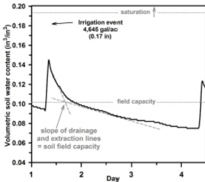
Figure 2. Example of practical determination of soil field capacity at 0-6 in. soil depth after irrigation event using soil moisture sensors.
