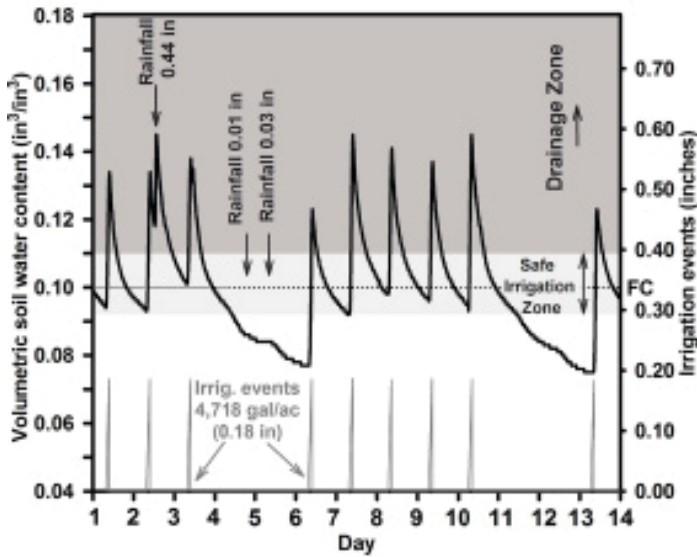
Figure 3. Example of excessive (“over”) irrigation of the upper soil layer (0- to 6-in. depth) moisture content for drip-irrigation under plastic mulched condition for sandy soils. Black line indicates volumetric soil water content using soil moisture sensors. Grey line indicates irrigation event, single daily irrigation event with volume application of 65 gal/100 ft (0.18 in). Dotted line indicates soil field capacity line. Arrows indicate rainfall events.
