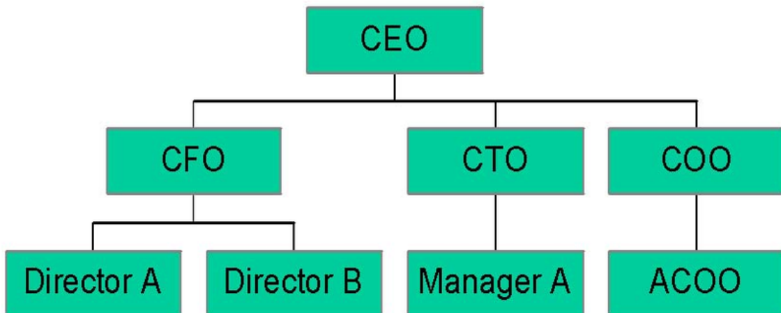
Figure 4.5 Tree
