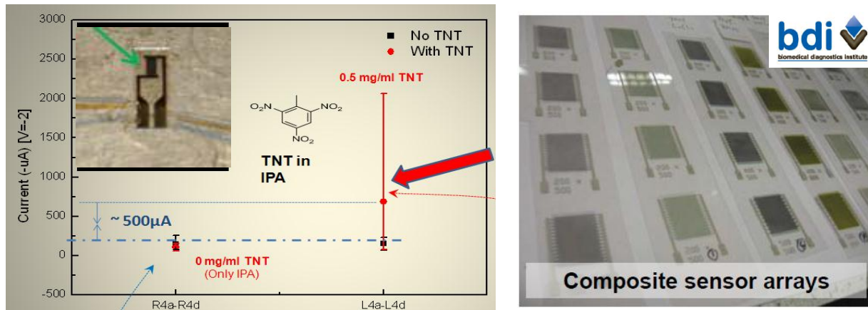
Figure 18 – Printed TNT Sensor shows resistance change in presence of explosives (Credit: Raptor Detection technologies). Chemical sensor array for NH 3 , H 2 S, CO, NO x , Cl 2 (Credit: Biomedical Diagnostics Institute).
