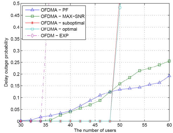
Figure 4. Delay outage probability in RT.
