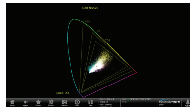
This CIE display is configured for 2020 colorspace with a 12G UHD SDI signal that has been constrained into a P3 colorspace.
