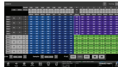
In this case a 12G signal has been applied to PRISM and shows each of the eight virtual streams. Line 41 was selected, and a search was performed to find the Start of Active Video (SAV).
