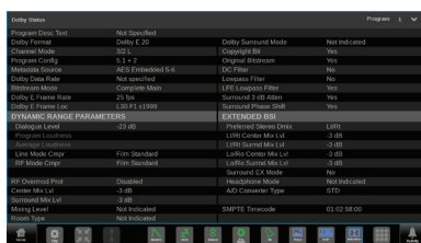
When Dolby E metadata is decoded the Dolby E Frame Location (Guardband) for the start of the metadata is shown within the display. The metadata shows the Dialnorm, Dynamic Range and Downmix parameters of the signal.
