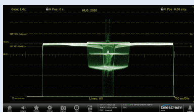
The gamma function on the input was configured for Hybrid Log Gamma (HLG) The input was then adjusted so that the 90% reflectance white and 18% grey level of the test scene were set at the appropriate levels.
