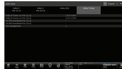
Dolby Timing tab shows Dolby E preamble location in SDI stream and location against house reference signal, BB or PTP.
