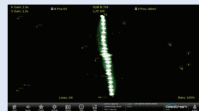
With a camera grey scale chart a deviation in the lower half of the display shows a red offset in the image.
