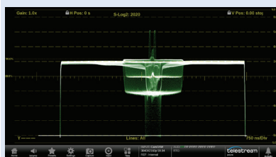
The Stop display is a logarithmic scale based on the input gamma transfer function that is configured. In this case S-Log 2 is setup as the gamma function and the Camera output was adjusted so that the 90% reflectance white and 18% grey levels were setup appropriately on the scale.
