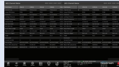
Using the flexible display configurations within PRISM a two-tile display each configured with AES Channel Status displays allows the user to scroll through the syntax information group by group. Allowing the user to easily compare AES Channel Status information for each group that can aid in troubleshooting issues.
