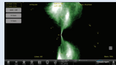
Gain and MAG adjustment allow for adjustment of color offset in the blacks at the center of trace.
