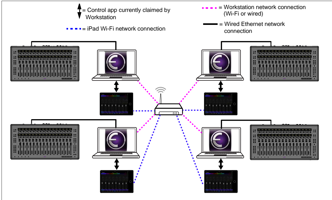
Multi-user environment example configuration
