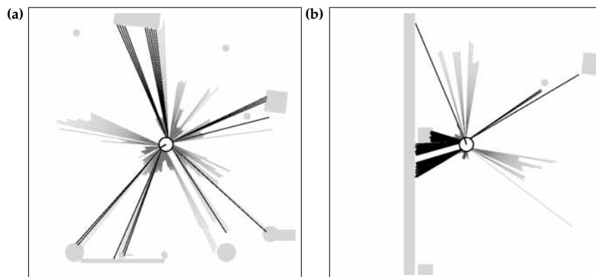
Figure 8.21 Laser range scans are often heavily corrupted when people surround the robot. How can a robot maintain accurate localization under such circumstances?
