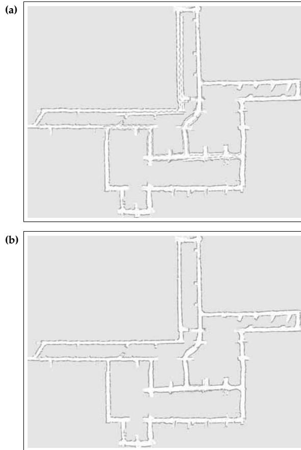
Figure 12.18 (a) Map with incremental ML scan matching and (b) full recursive branch-and-bound data association. Images courtesy of Dirk Hähnel, University of Freiburg.
