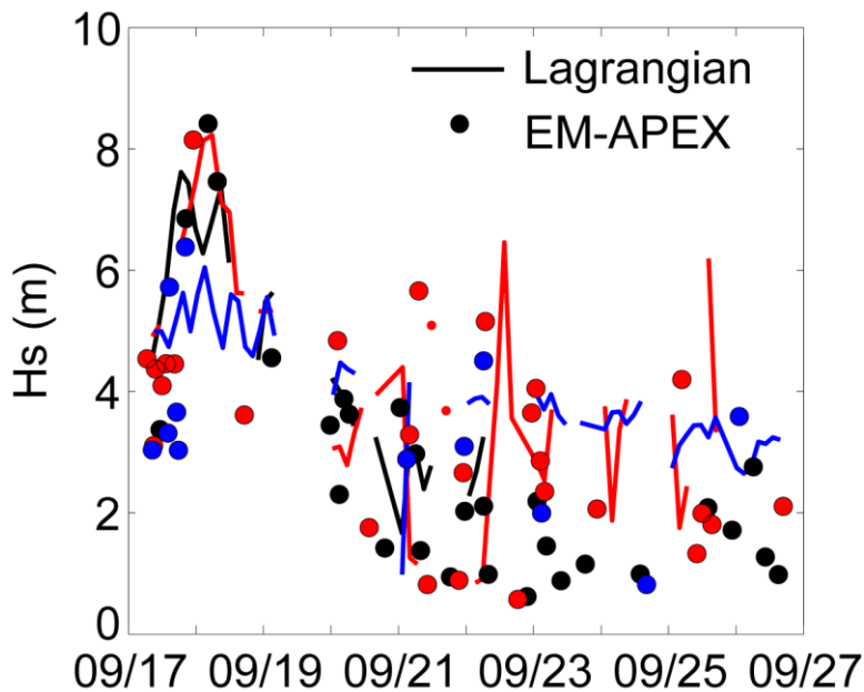
Figure 3. Significant wave height from EM-APEX floats (dots) and Lagrangian floats (lines) in Typhoon Fanapi. Floats of the same color were deployed together.
