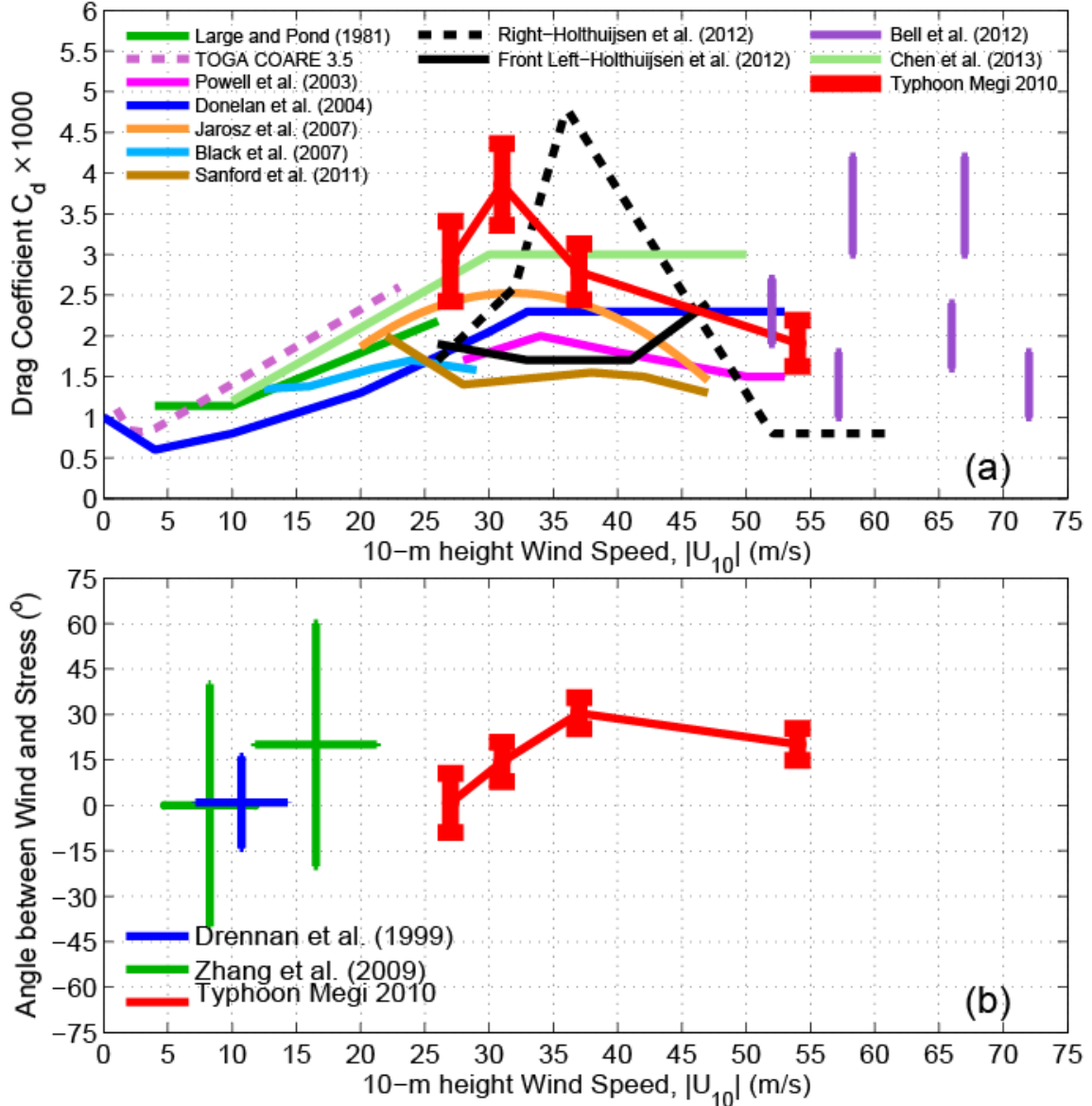
Fig. 1. (a) Parameterization of drag coefficient C_d as a function of wind speed at 10 m above the sea surface, |\overline{U}_{10}| , including Large and Pond (1981), TOGA COARE bulk algorithm 3.5 (Edson et al. 2013), Powell et al. (2003), Donelan et al. (2004), Jarosz et al. (2007), Black et al. (2007), Sanford et al. (2011), Holthuijsen et al. (2012), Bell et al. (2012), and Chen et al. (2013). (b) Previous estimates of the orientation difference between the surface wind and stress vectors. Values taken from Fig. 6 in Drennan et al. (1999), and Figs. 1 and 3 in Zhang et al. (2009) are plotted. Measured wind speed in Drennan et al. (1999) and Zhang et al. (2009) is extrapolated to 10 m above sea surface by assuming a logarithmic wind profile in the vertical. The horizontal and vertical bars describe the ranges of their data. The positive angle represents that the stress vector points clockwise from the wind vector.
