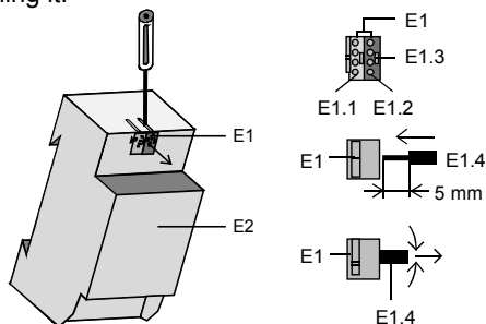
Figure 4: Connecting and disconnecting bus wires
