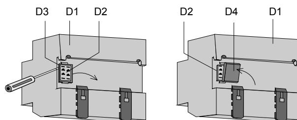
Figure 3: Insulation of the contact system
