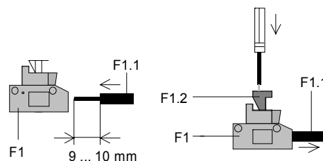
Figure 5: Connecting and disconnecting load circuits
