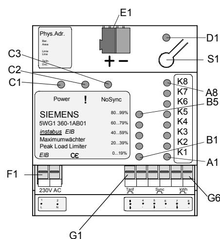
Figure 1: Location of the display and operator elements
