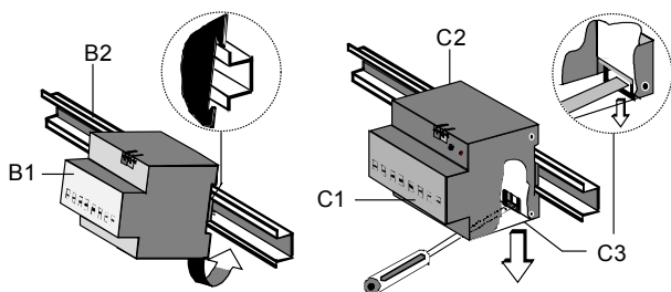
Figure 2: Mounting and dismounting a DIN-rail device
