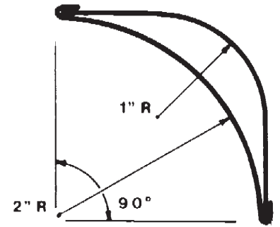
108 2" Double Wall Vane
