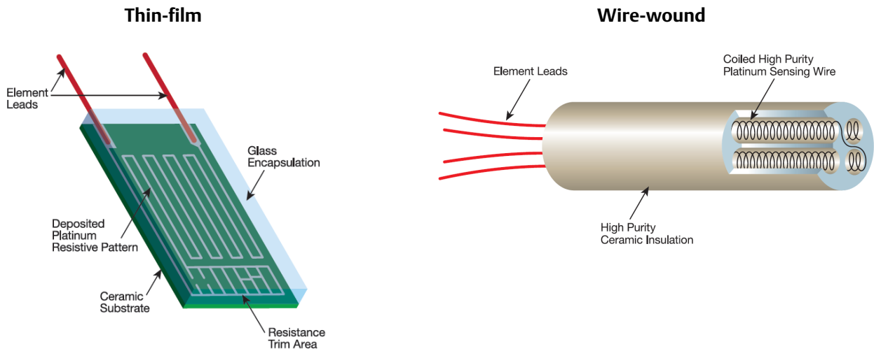
Figure 3. RTD Elements
