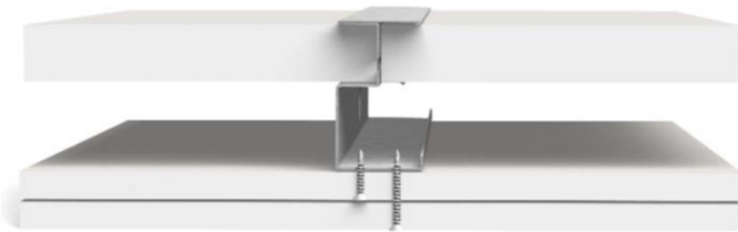
Shaftwall
