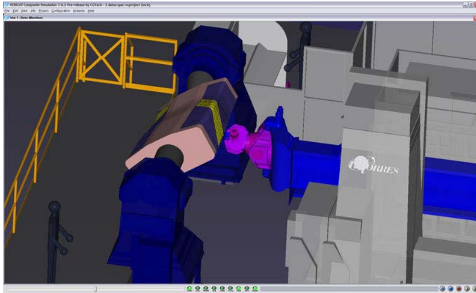
Figure 8 – An mTorres AFP machine creating two spars on one tool
