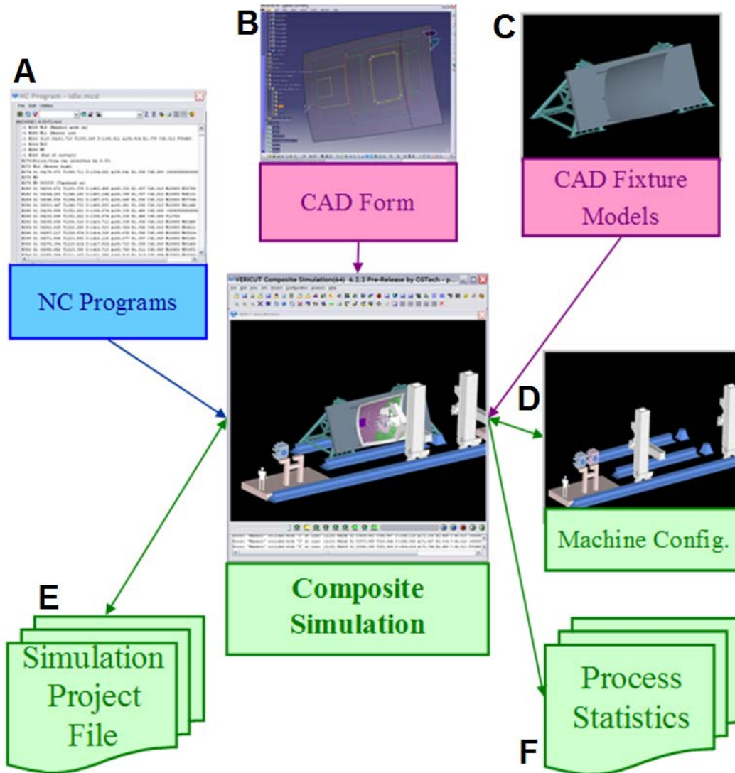
Figure 4. Overview of AFP Simulation Software
