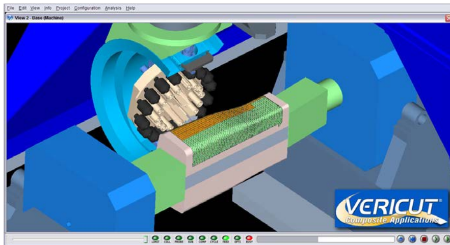
Figure 7 – Current programming and simulation project involving an Electroimpact gantry design with removable rotisserie.
