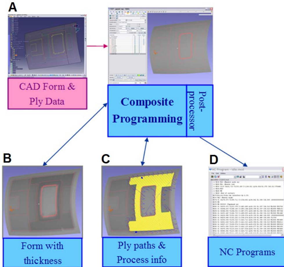
Figure 2. AFP programming software overview
