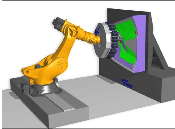
Figure 10 – A simulation rendering of a Kuka robot with Electroimpact AFP head.
