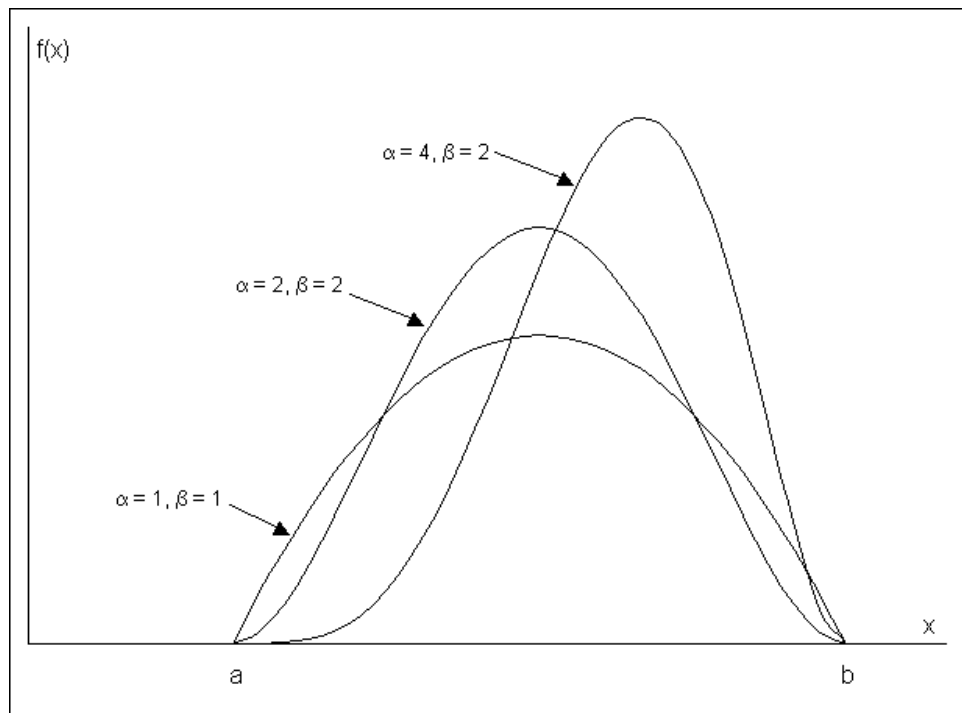
Figure 11-1 Illustration of Several Beta Distributions
