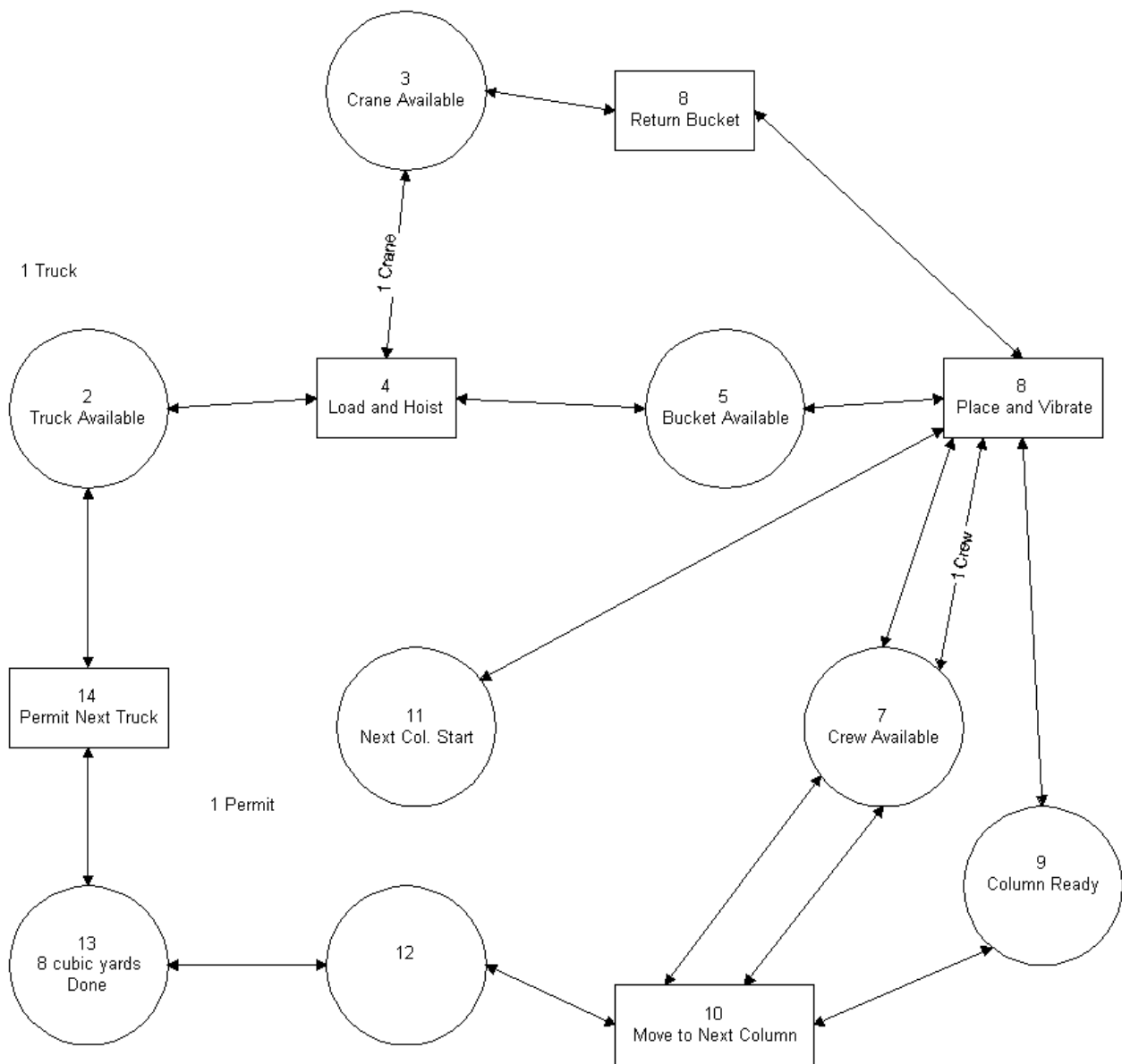
Figure 4-5: Illustration of a Concrete-Placing Simulation Model
