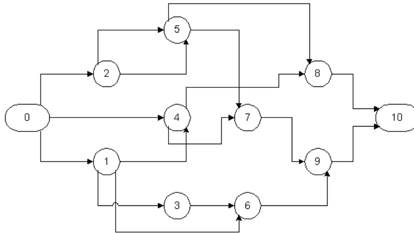
Figure 10-15 Example Project Network with Lead Precedences
