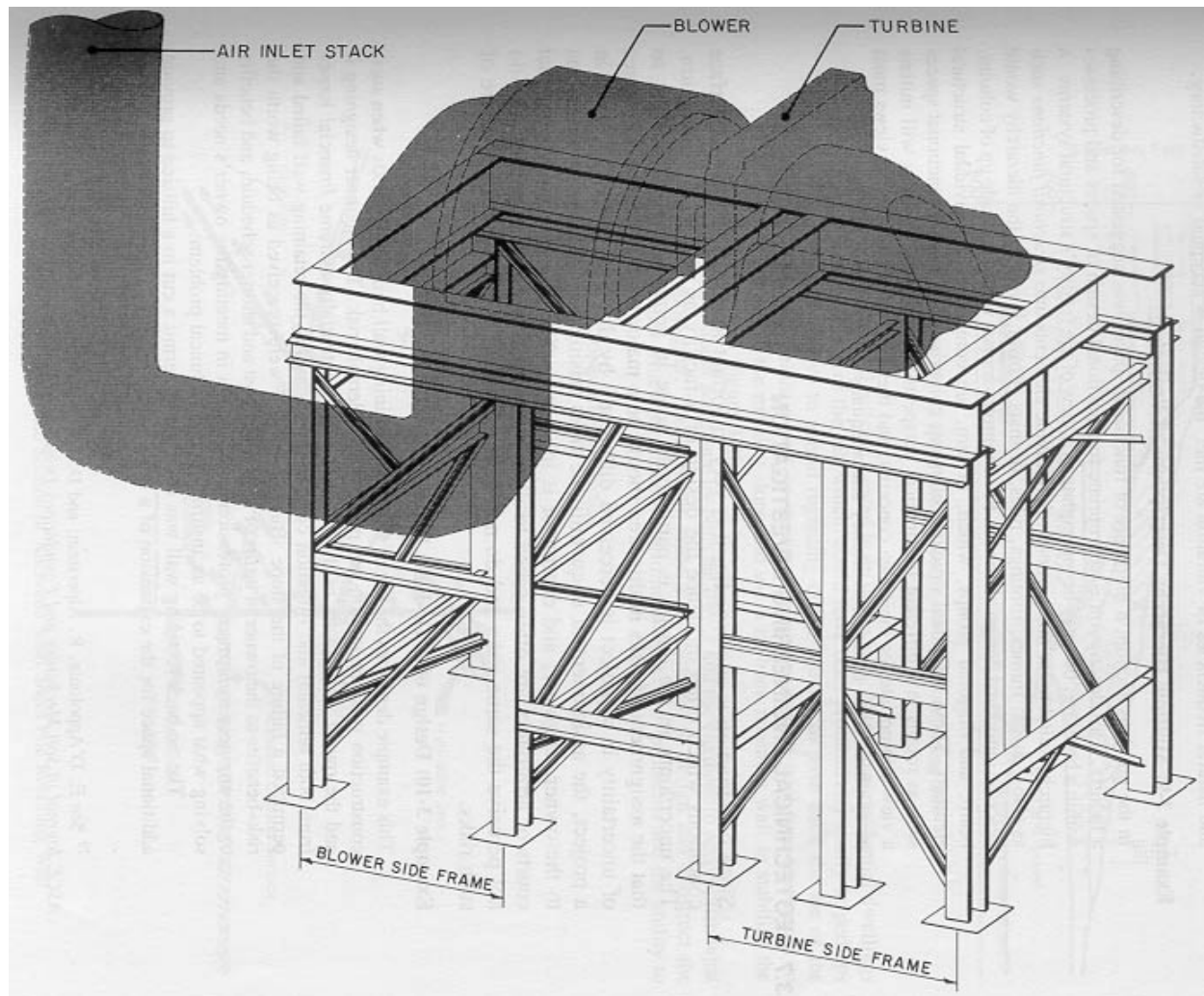
Figure 3-8: Steel Frame Supporting a Turbo-Blower
