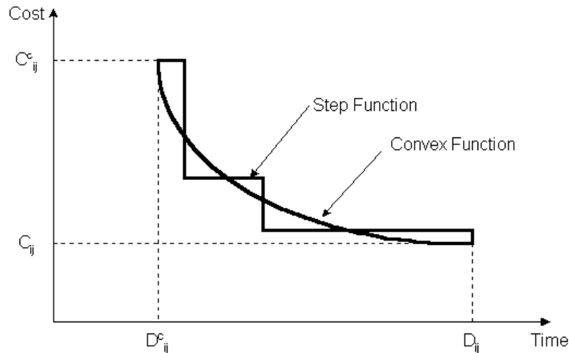
Figure 11-4 Illustration of Non-linear Time/Cost Tradeoffs for an Activity
