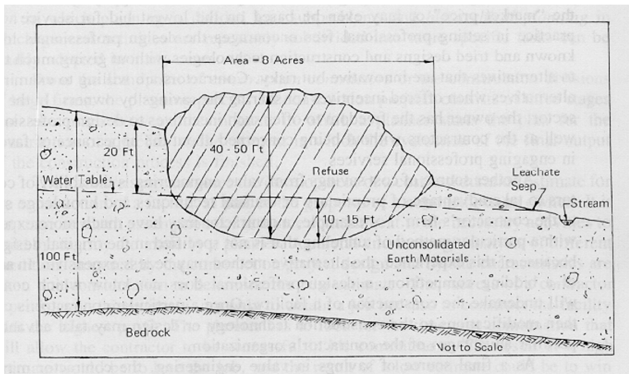
Figure 3-11: Cross-Section Illustration of a Landfill
