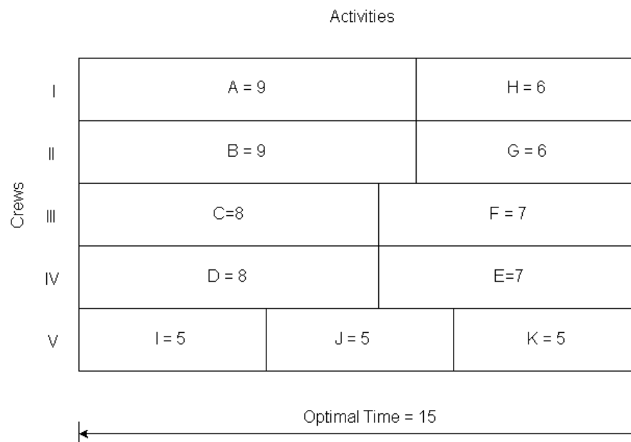
Figure 10-16 Example Allocation of Crews to Work Tasks
