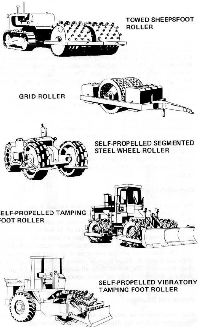
Figure 4-4 Some Major Types of Compaction Equipment
