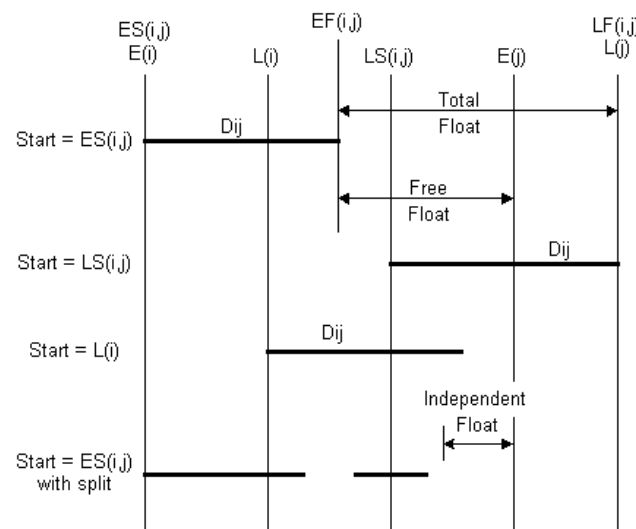
Figure 10-6 Illustration of Activity Float
