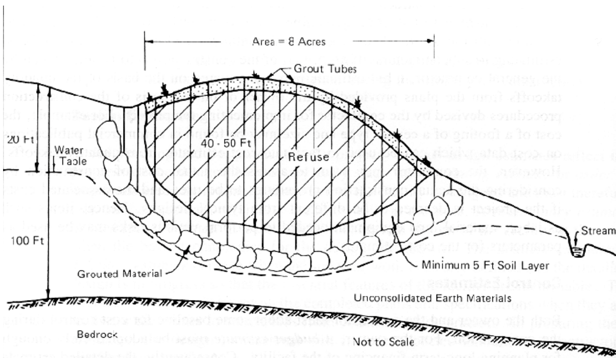
Figure 5-1: Grout Bottom Seal Liner at a Landfill
