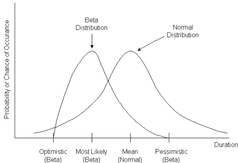
Figure 9-9 Beta and Normally Distributed Activity Durations
