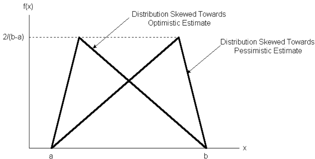
Figure 11-2 Illustration of Two Triangular Activity Duration Distributions
