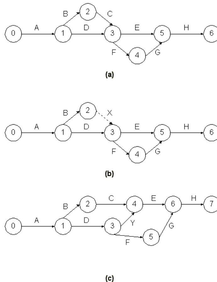
Figure 10-1 Dummy Activities in a Project Network
