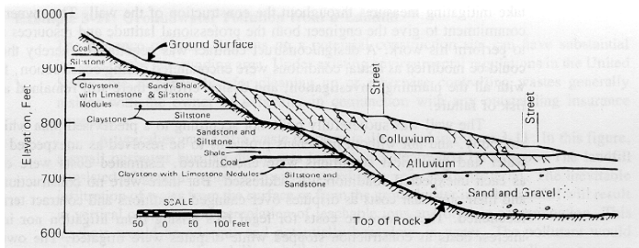
Figure 3-9: Typical Cross Section of Hillside Adjoining Site
