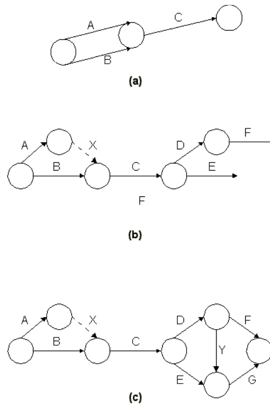
Figure 10-2 An Activity-on-Branch Network for Critical Path Scheduling
