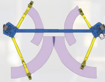
CONVENTIONAL 2-STAGE ARMS with FLIP-UP ADAPTERS
