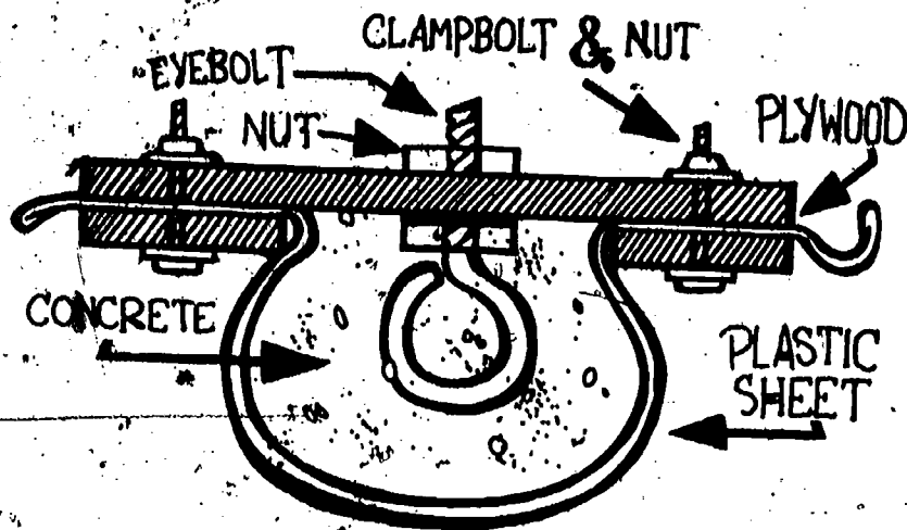
Figure 30: The plastic-sheet-plywood molding method.
