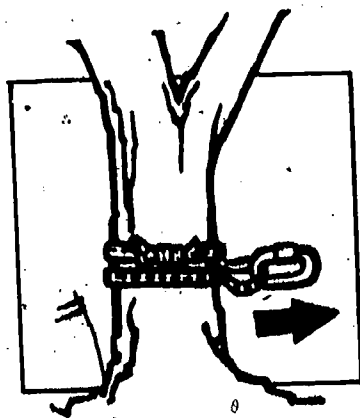
Figure 28: Using a tree, "loops" or "runners", and a locking carabiner to form an anchor.
