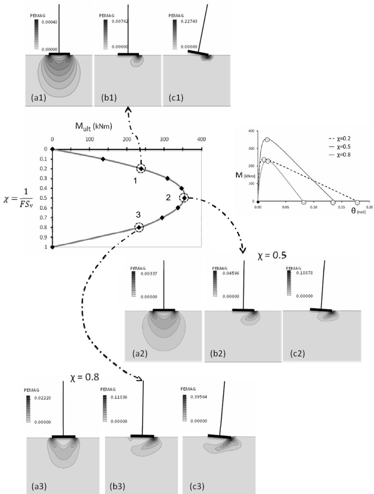
Fig. 2. Dependence of the moment capacity of the foundation on the static safety factor FS_v ( M - \chi diagram). For the three cases (1,2,3), corresponding to values of \chi 0.2, 0.5, 0.8, we display three snapshots of the deformed system along with the contours of plastic deformation. Specifically a1,a2,a3 present the initial (static) state; b1,b2,b3 present the states at the peak moment, M_{ult} = 238, 354, 232 kNm, respectively; c1, c2, c3 show the states of imminent collapse. Also shown are the M - \theta pushover curves for the three \chi values.
