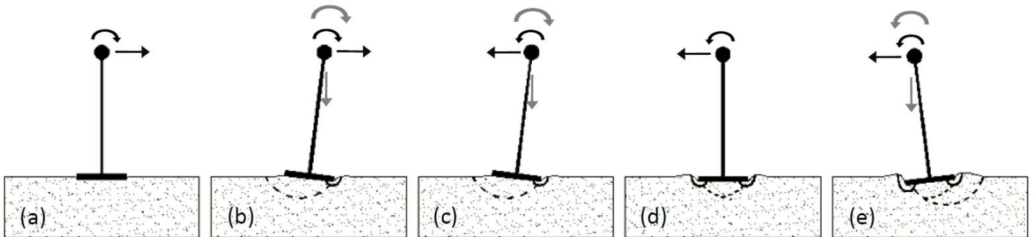
Fig. 6. Schematic snapshots of the displacement / rotation of the system and the corresponding bearing capacity failure mechanisms.
