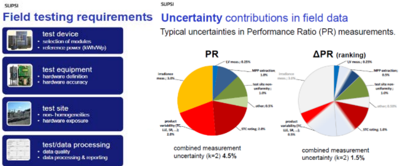
Figure 63: Field testing requirements and contributions to uncertainty in outdoor PV module yield measurements.
