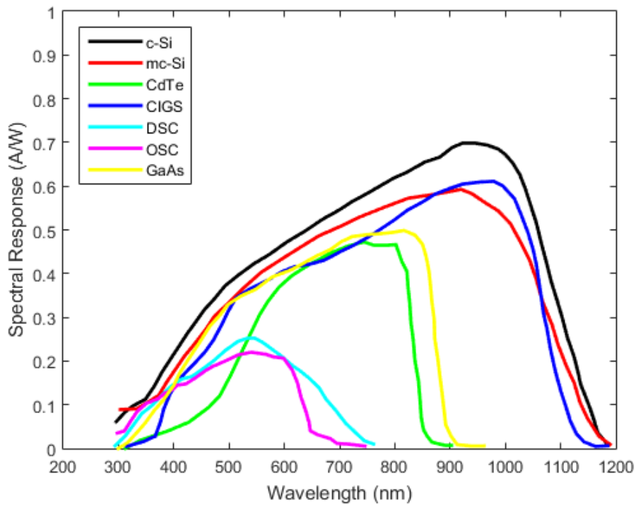
Figure 6: Representative spectral response curves for typical PV cell technologies from the PVPIC website [13]).
