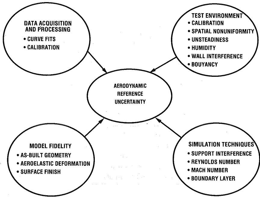
Fig. 1.2 Contributions to Aerodynamic Reference Uncertainty.
