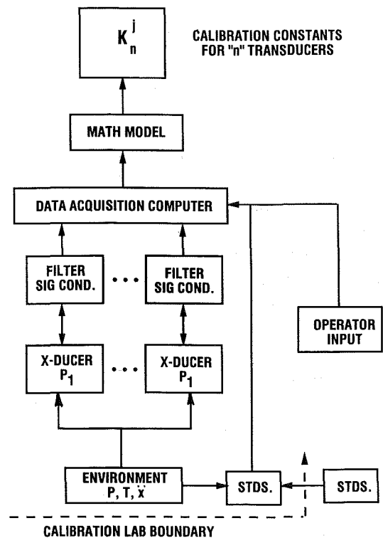
Fig. 3.3 Calibration of pressure transducers.
