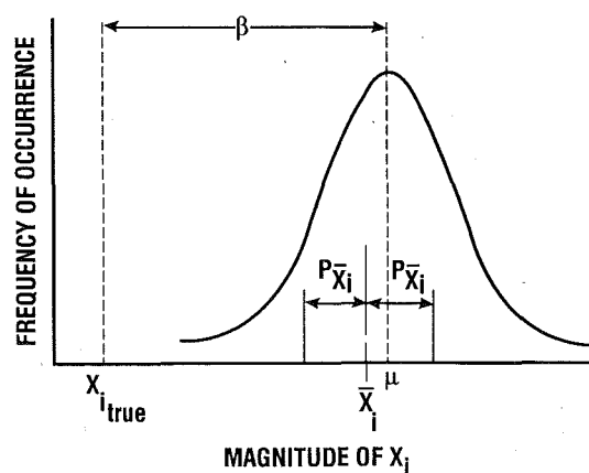
Fig. 2.5 95-percent confidence precision limit interval around the mean value of a sample of readings of variable X_i .
