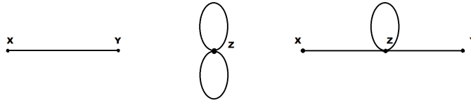
Figure 2.3: First and second term of \mathcal{O}(\lambda^1) .
