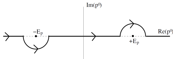
Figure 1.3: Contour C of the Feynman propagator.
