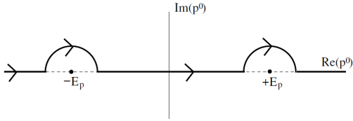
Figure 1.5: The retarded contour.
