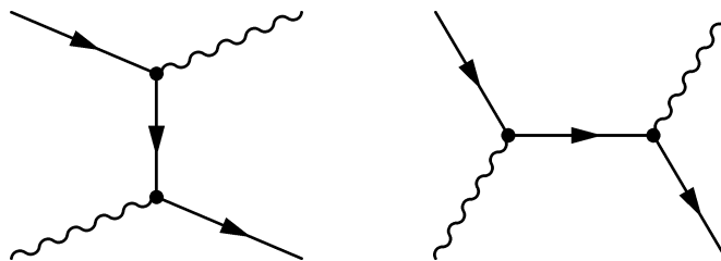
Figure 4.4: Compton scattering at leading order.
