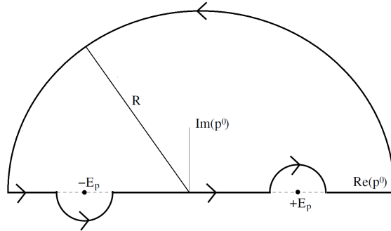
Figure 1.2: Contour C_2 .
