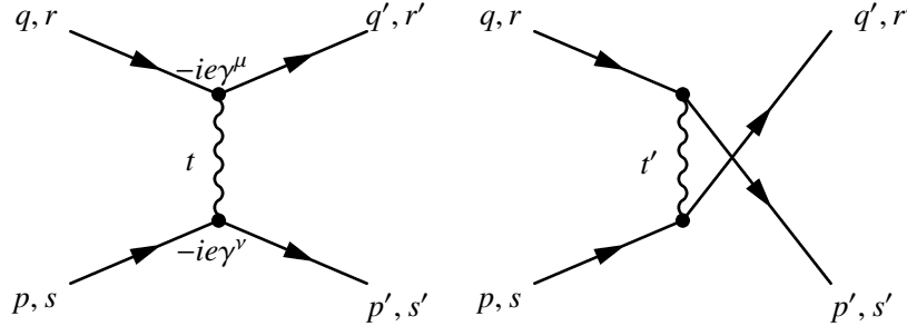
Figure 4.1: Leading order Feynman diagrams for electron scattering.
