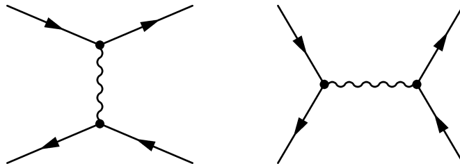
Figure 4.3: Bhabha scattering at leading order.
