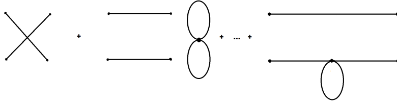
Figure 2.4: Diagrams for \lambda^1 .
