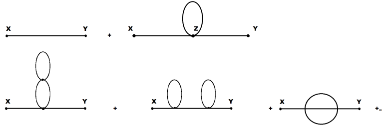
Figure 2.5: Perturbative corrections.
