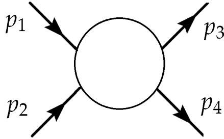
Figure 2.9: 2 – 2 scattering.
