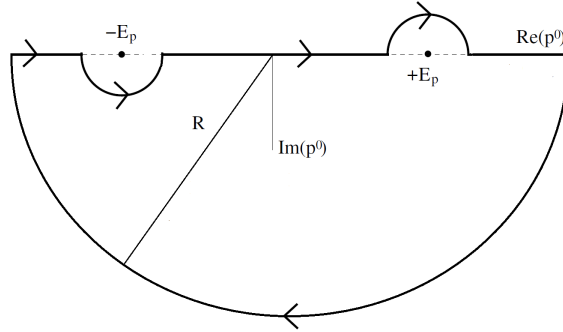
Figure 1.1: Contour C_1 .
