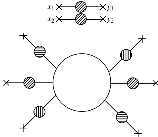
Figure 2.7: Partially connected diagram, i.e. (n-2) and (r-2) .
