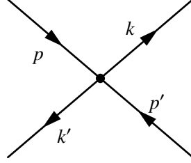
Figure 5.2: Centre-of-mass frame, p in \hat{z} -direction.
