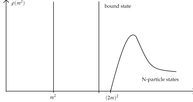
Figure 2.1: Spectral function.
