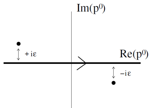
Figure 1.4: Shifted poles.
