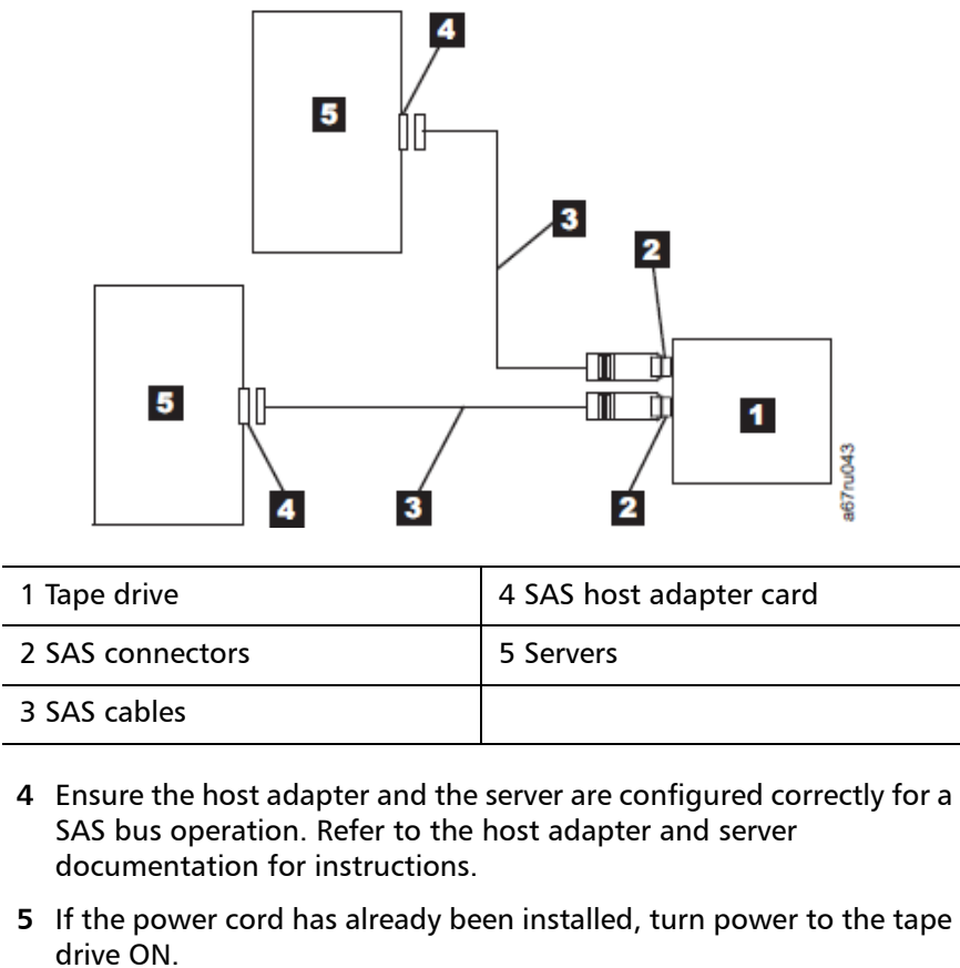
Figure 6 Example of connecting the SAS device to two servers
