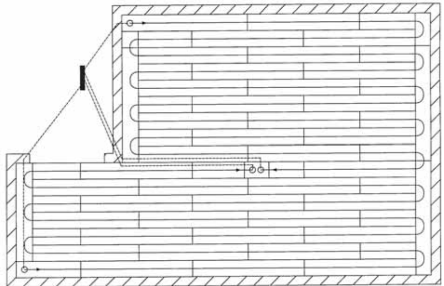
Figure 8: Manifold Location in the Joist Cavity
