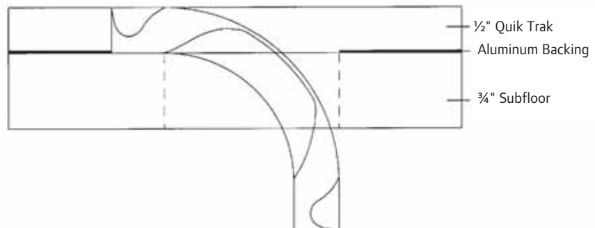
Figure 20: Trim Aluminum Backing to Allow Bend Support to be Flush with the Top of the Panels
