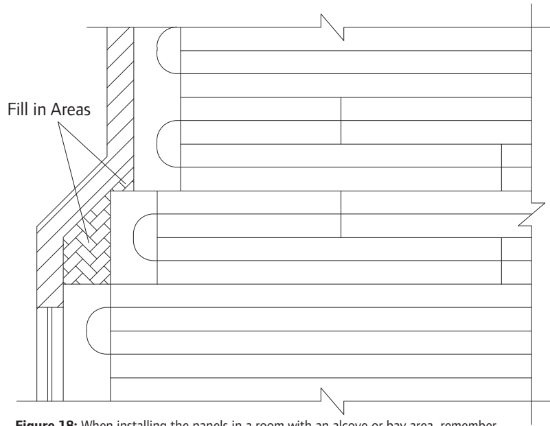
Figure 18: When installing the panels in a room with an alcove or bay area, remember to allow enough room for the Return Trak panels. Fill any areas not covered with panels with 1/2" plywood.
