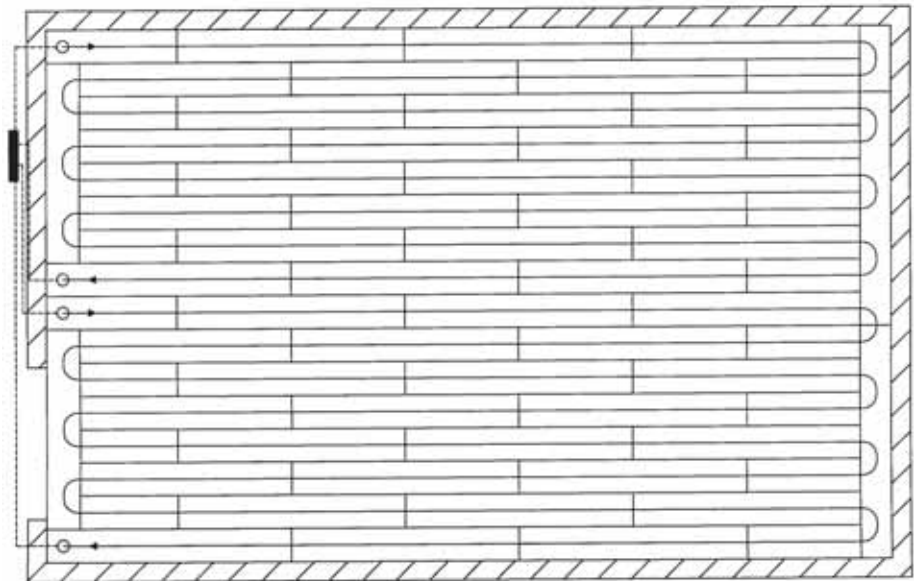
Figure 7: Manifold Location in the Joist Cavity
