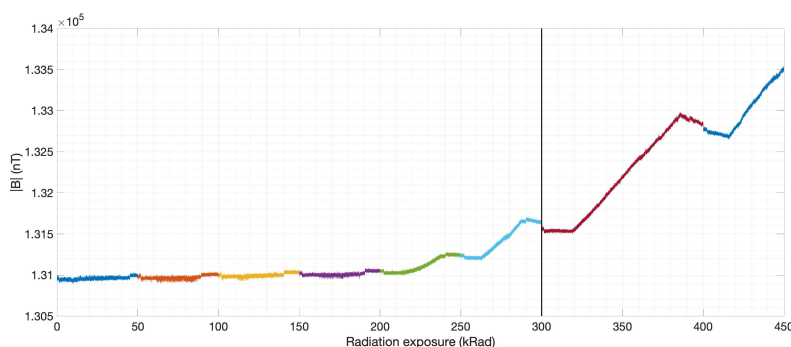
Figure 6. Magnetic field magnitude measured during the radiation tests at the Department of Nuclear Engineering and Radiological Sciences at the University of Michigan.
