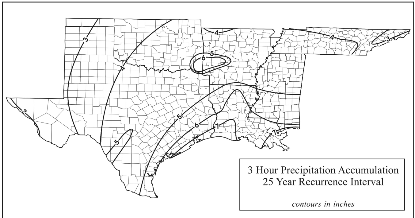
Fig. 3.4. 3-hour 25-year rainfall pattern
