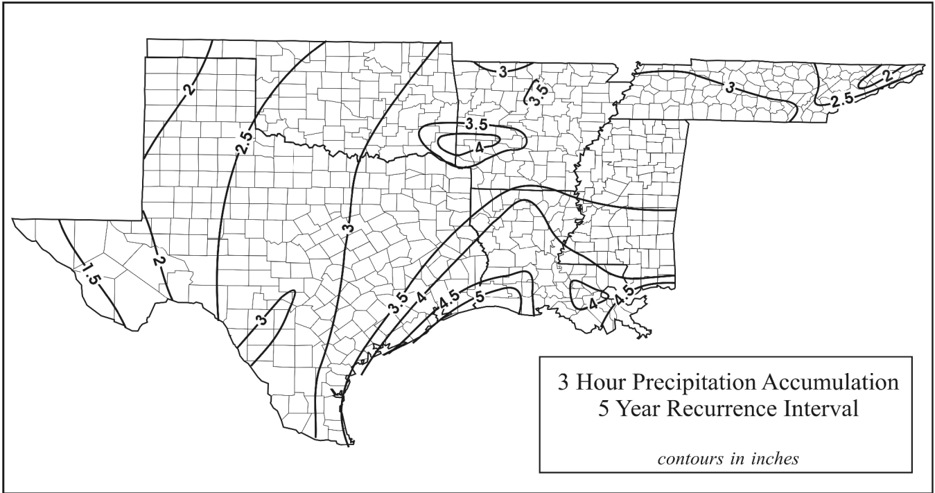
Fig. 3.2. 3-hour 5-year rainfall pattern.
