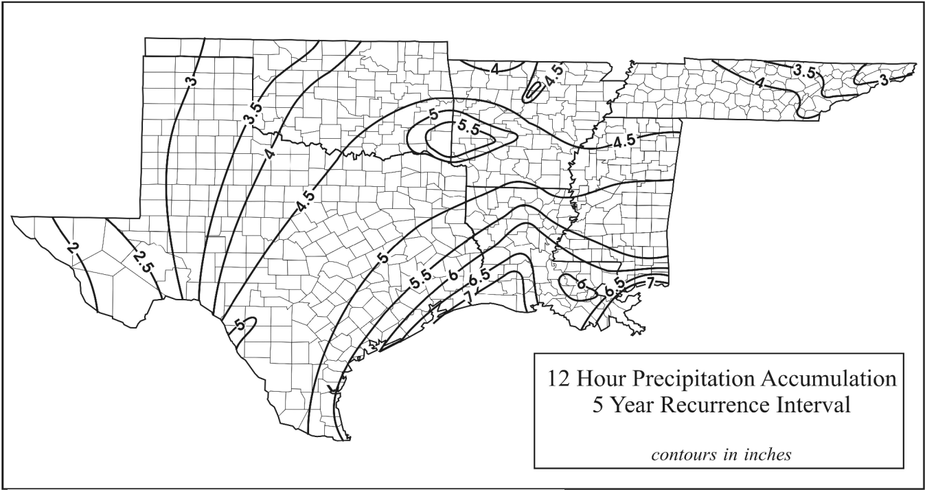
Fig. 5.2. 12-hour 5-year rainfall pattern
