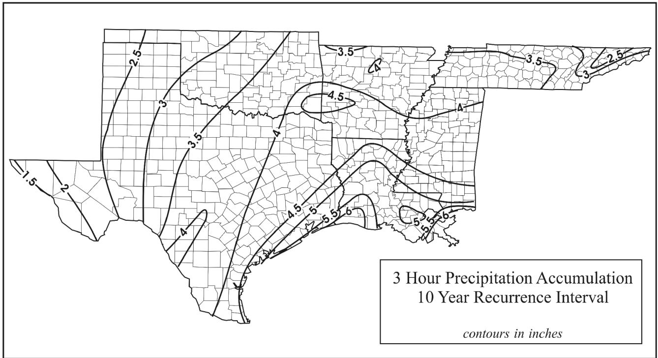
Fig. 3.3 3-hour 10-year rainfall pattern.
