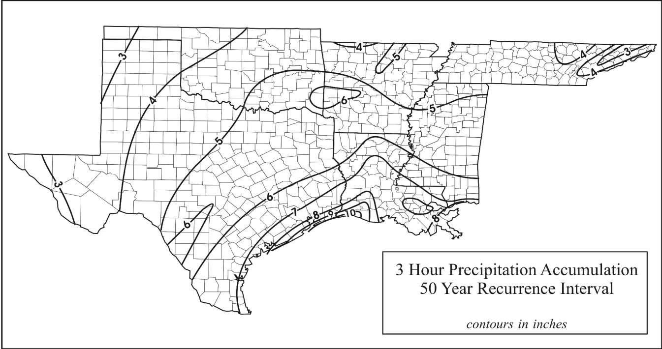
Fig. 3.5. 3-hour 50-year rainfall pattern.
