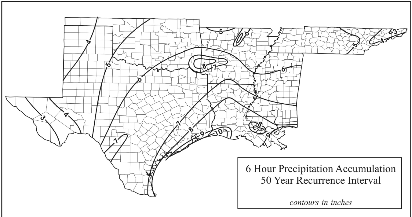
Fig. 6-hour 50-year rainfall pattern.
