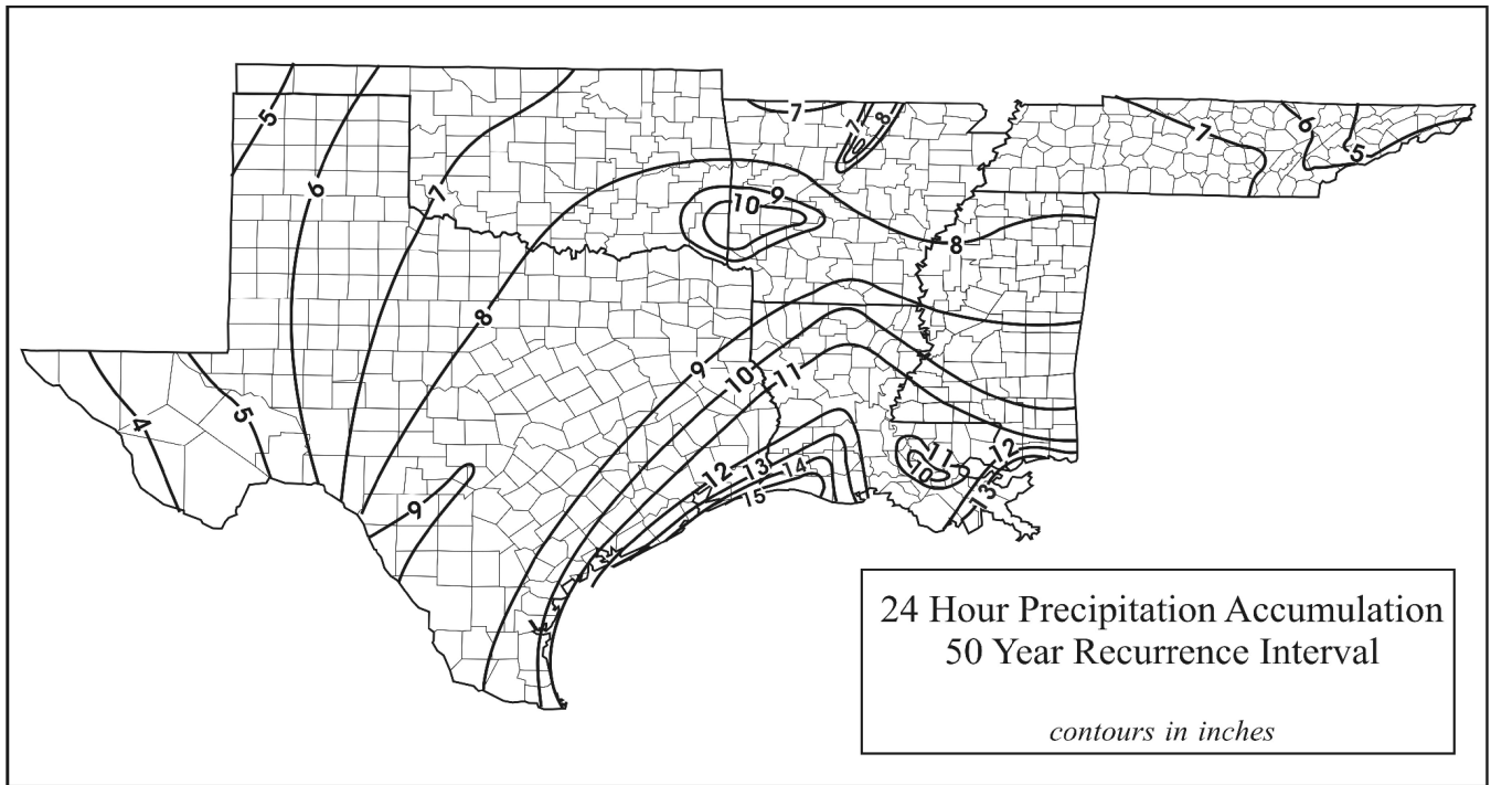
Fig. 6.5. 24-hour 50-year rainfall pattern.
