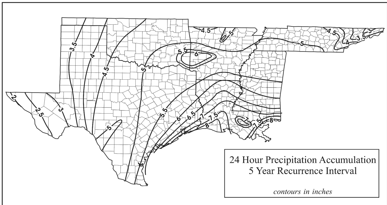
Fig. 6.2. 24-hour 5-year rainfall pattern.
