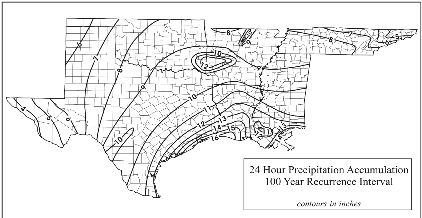
Fig. 6.6. 24-hour 100-year rainfall pattern.
