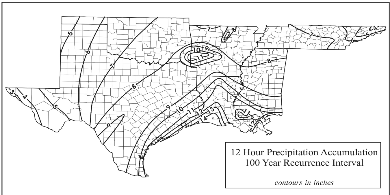
Fig. 5.6. 12-hour 100-year rainfall pattern.
