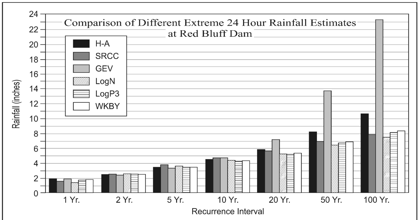
Fig. 10. Quantile estimates of 24-hour storms at Red Bluff Dam, Texas.
