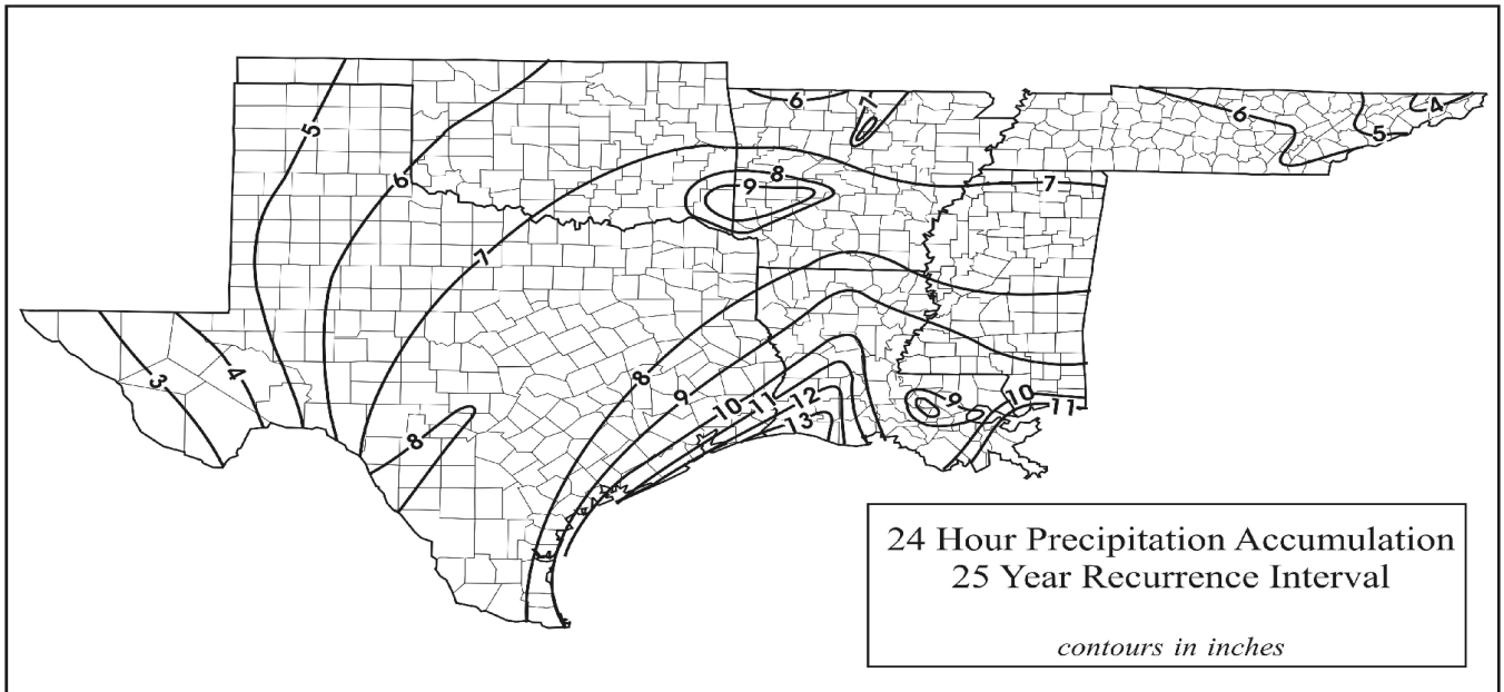
Fig. 6.4. 24-hour 25-year rainfall pattern.
