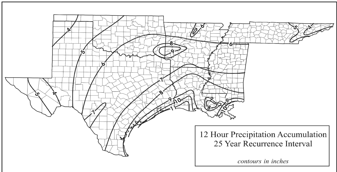
Fig 5.4. 12-hour 25-year rainfall pattern.
