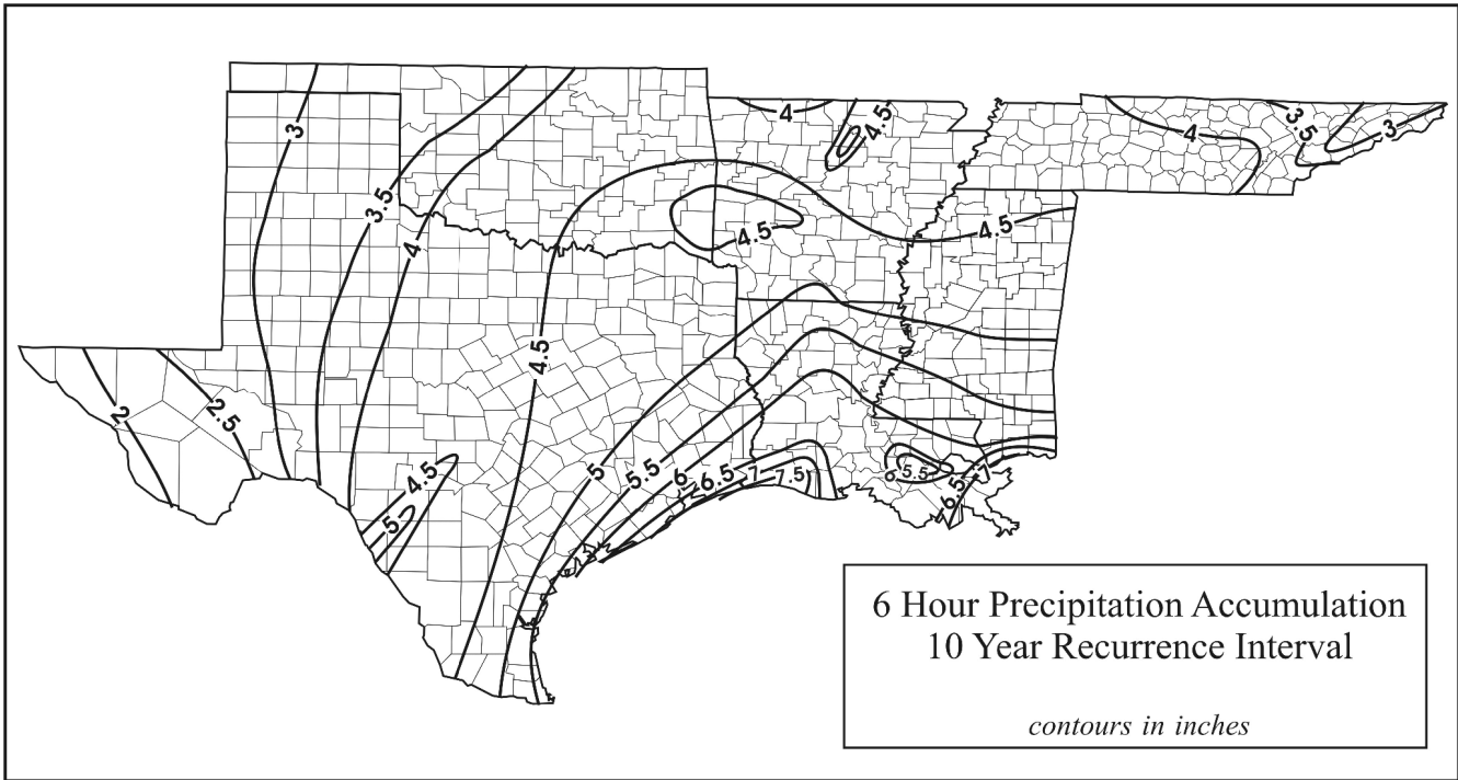
Fig. 4.3. 6-hour 10-year rainfall pattern
