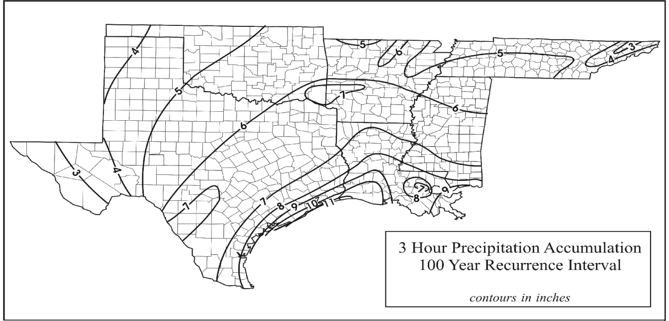
Fig. 3.6. 3-hour 100-year rainfall pattern.
