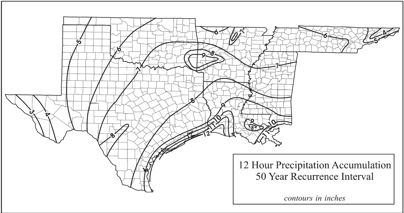
Fig. 5.5. 12-hour 50-year rainfall pattern.
