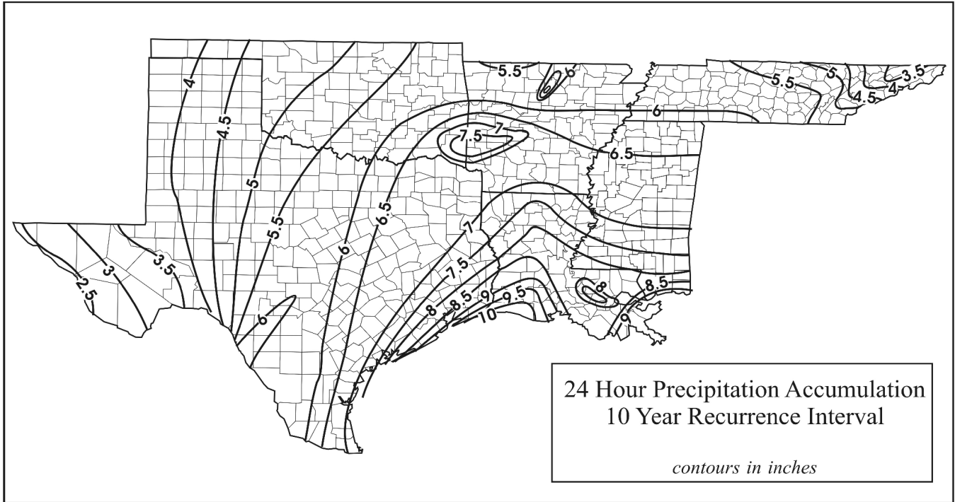
Fig. 6.3. 24-hour 10-year rainfall pattern.
