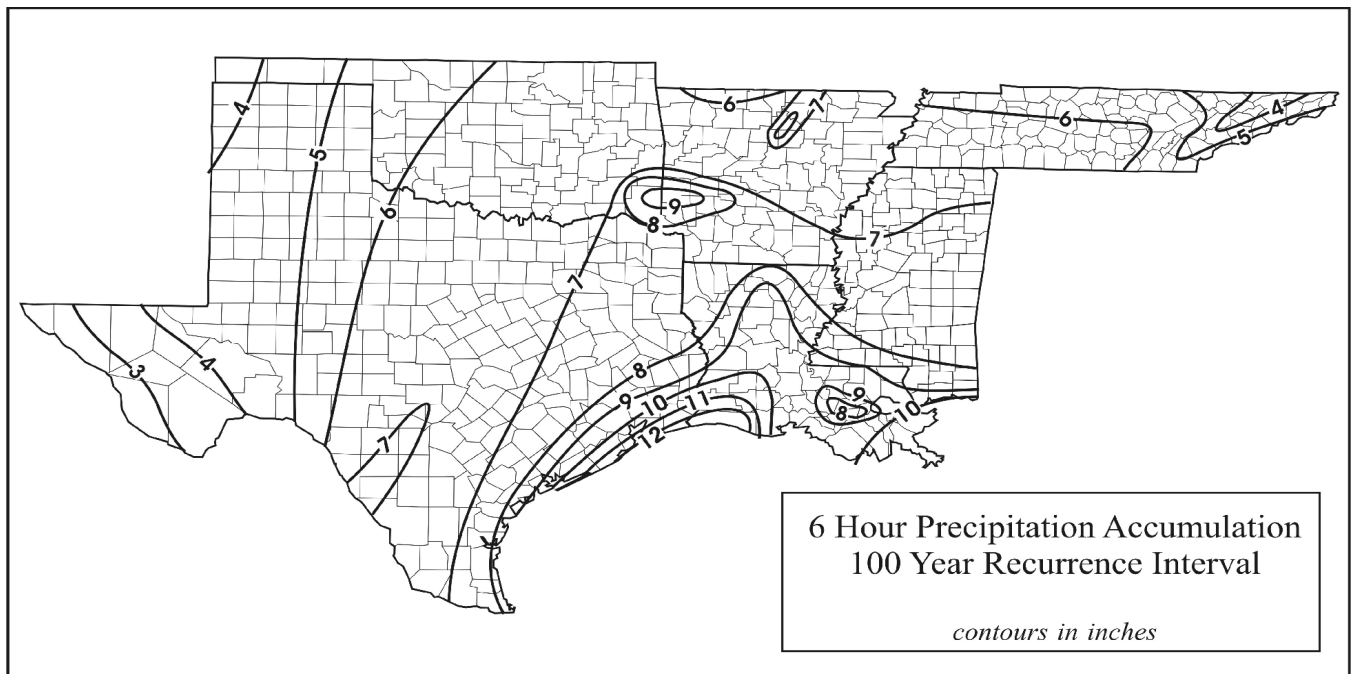
Fig. 4.6. 6-hour 100-year rainfall pattern.
