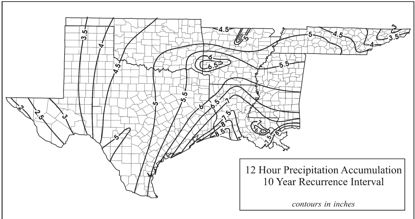
Fig. 5.3. 12-hour 10-year rainfall pattern.
