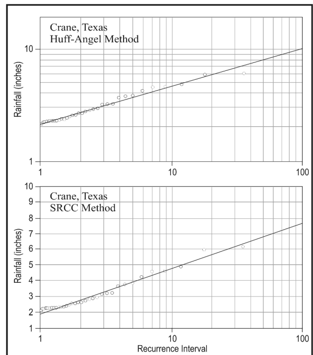
Fig. 9. Quantile estimates of storm rainfall for Crane, Texas, by the Huff-Angel and SRCC methods.
