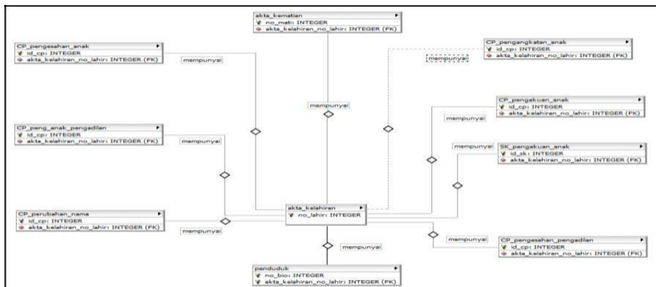
Gambar 6. Entity Relationship Diagram 3
