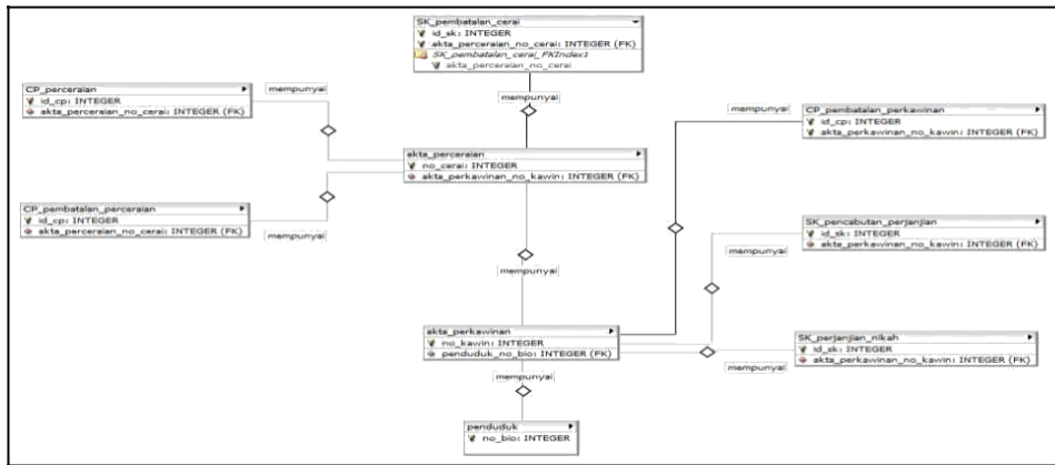
Gambar 7. Entity Relationship Diagram
