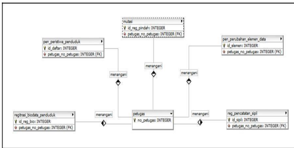
Gambar 4 Entity Relationship Diagram 1
