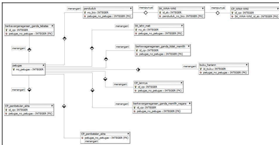
Gambar 4 Entity Relationship Diagram 1
