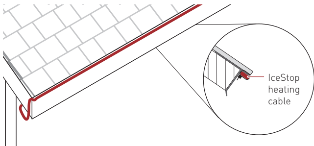
Figure 9: Layout for heated drip edge
