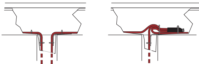
Figure 22: GM-RAKE downspout hangers
