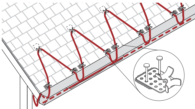
Figure 16: GMK-RC mechanical attachment
