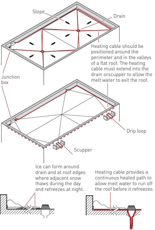
Figure 7: Layout on a flat roof
