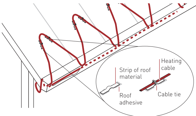
Figure 19: Belt loop approach on a sloped roof
