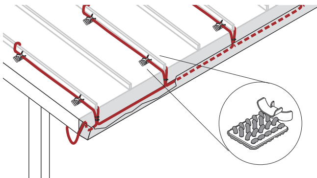
Figure 17: GMK-RC adhesive attachment
