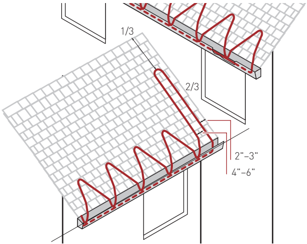
Figure 11: Layout for a roof/wall intersection
