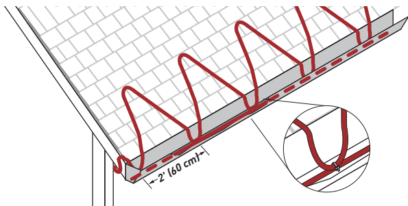
Figure 5: Layout in a zig-zag pattern
