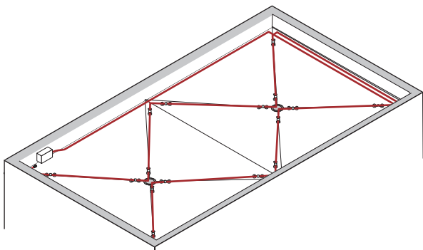
Figure 20: Belt loop approach on a flat roof
