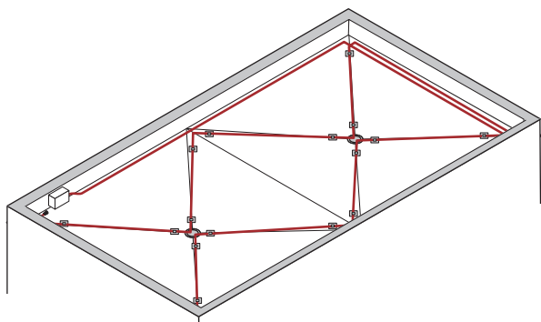
Figure 18: GMK-RC clip on flat roof
