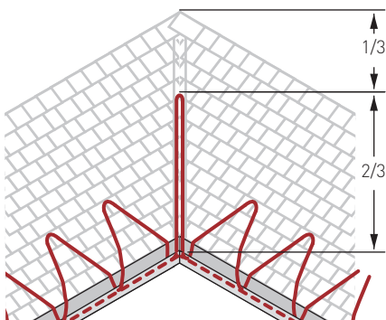
Figure 10: Layout for a roof valley
