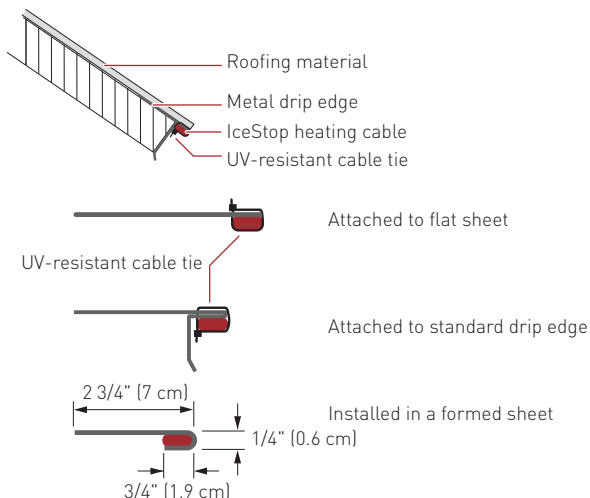
Figure 23: Heated drip edge attachment guidelines
