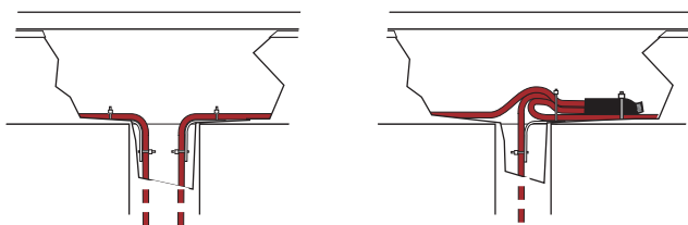
Figure 14: Heating cable at top of downspout
