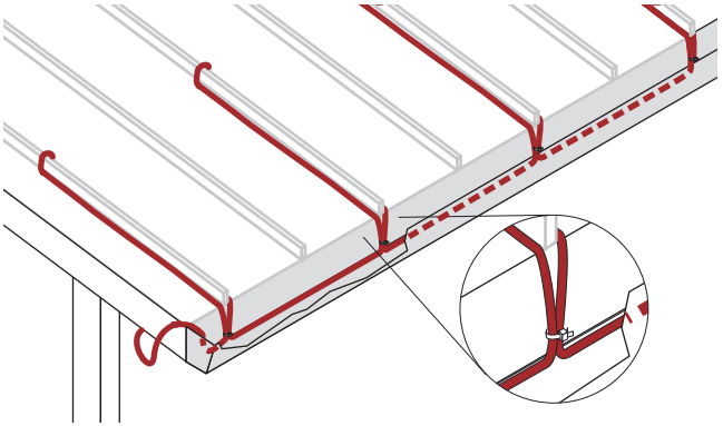
Figure 6: Layout on a standing seam roof
