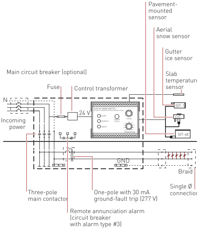
Figure 26: Typical wiring diagram of group control with SMPG1
