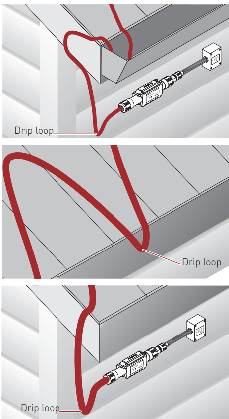
Figure 24: Drip loops
