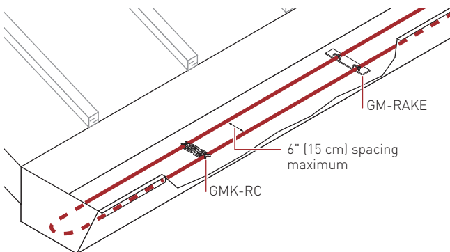
Figure 21: GMK-RC clip on a gutter
