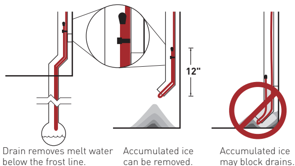
Figure 15: Heating cable at bottom of downspout
