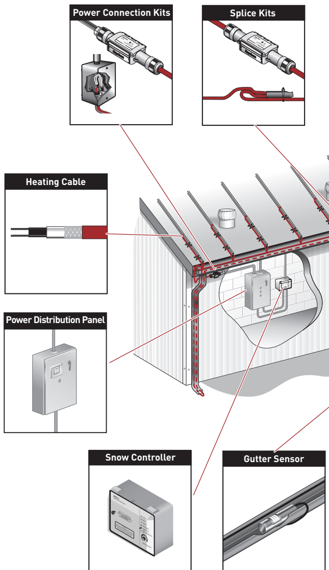
Figure 1: IceStop Roof and Gutter De-icing System
