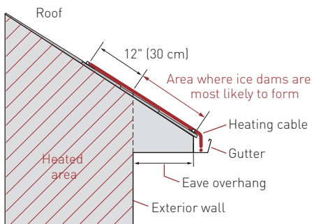
Figure 4: Side view of roof with IceStop system
