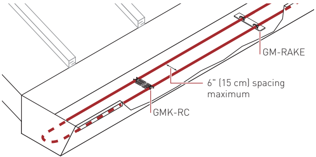
Figure 13: Layout in wide gutters—6" to 12" wide
