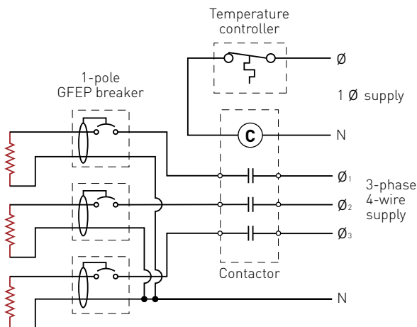
Figure 25: Typical controller wiring—multiple circuits
