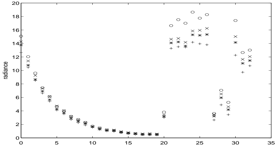
Fig. 17. Lamp 2 calibration data. The first 20 points are the measured radiance from gray strips on the Kodak standard card. The last 13 points are the measured radiance from the 18% gray card followed by the 12 color strips on the Kodak standard card. The lamp calibration was repeated four times on separate days. Data from the first, second, third and fourth calibrations are plotted with the symbols 'o', 'x', '*' and '+' respectively. Notice a small decrease in the lamp brightness with time.
