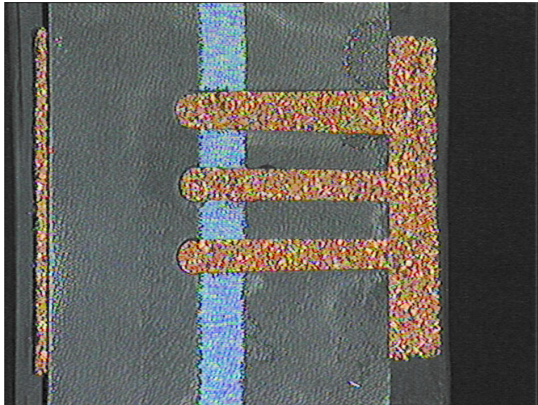
Fig. 8. Fiducial Marker attached to Sample. This metallic grid with painted stripe is used as a fiducial marker to specify a spatial region for measuring radiance with the photometer and recording pixel values with the video camera. These radiance and pixel measurements are used in radiometric calibration.
