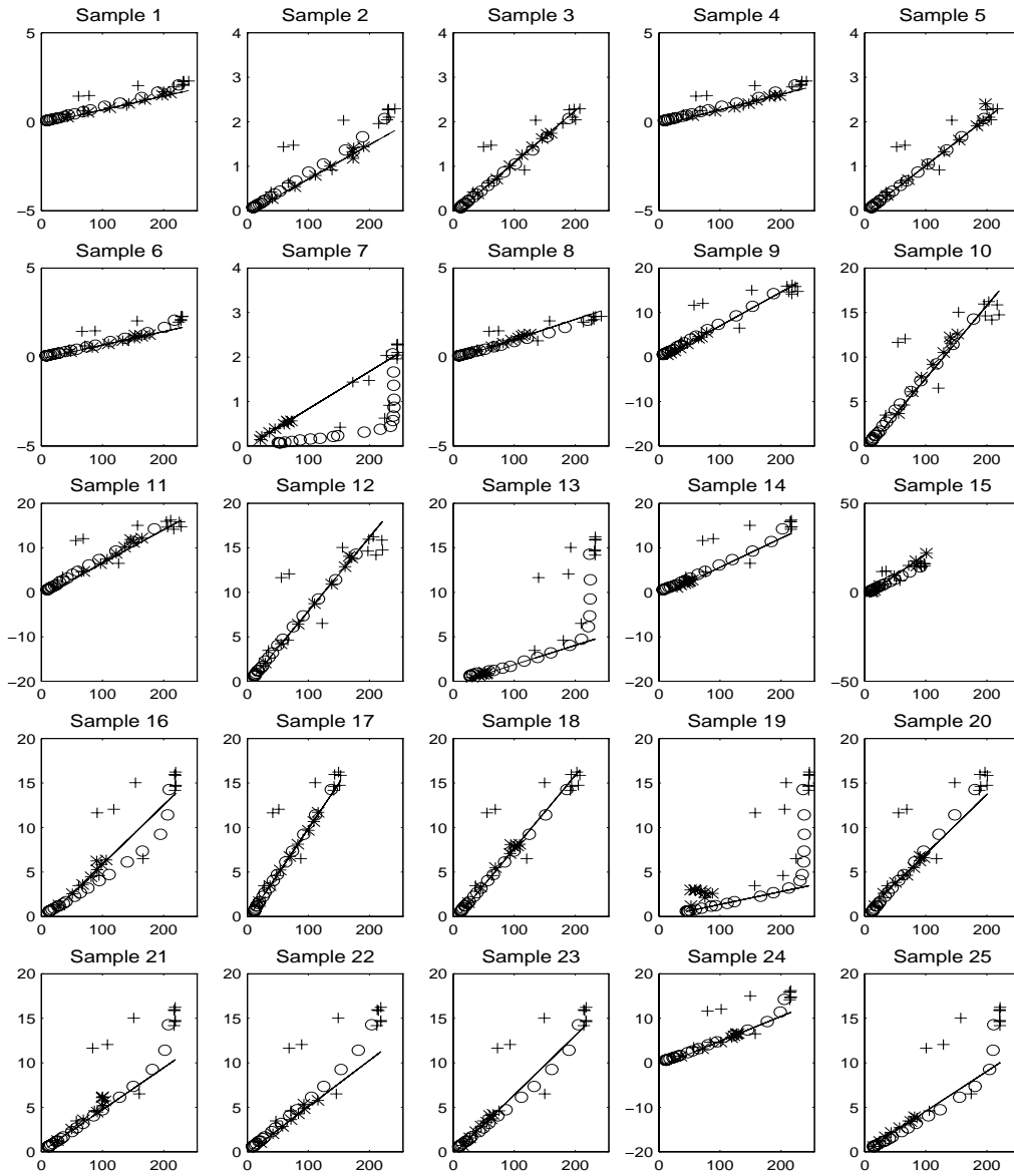
Fig. 19. Calibration plots for the gray calibration data for samples 1-25. The plots show pixel value (abscissa) and radiance measured by the photometer (ordinate). The sample calibration data are plotted with the symbol “*”. The gray strips from the standard calibration data are plotted with the symbol “o”, and the colored strips from the standard calibration data are plotted with the symbol “+”. The estimated linear calibration function is plotted with a solid line. Figure 20 uses the same plotting symbols.
