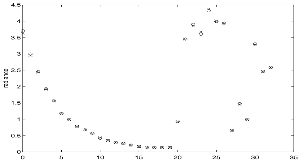
Fig. 18. Lamp 3 calibration data. The first 20 points are the measured radiance from gray strips on the Kodak standard card. The last 13 points are the measured radiance from the 18% gray card followed by the 12 color strips on the Kodak standard card. The lamp calibration was repeated twice on separate days. Data from the first set is plotted with the symbol 'o'. Data from the second set is plotted with the symbol 'x'.
