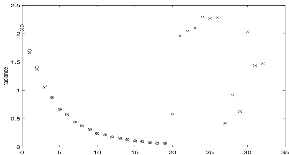
Fig. 16. Lamp 1 calibration data. The first 20 points are the measured radiance from gray strips on the Kodak standard card. The last 13 points are the measured radiance from the 18% gray card followed by the 12 color strips on the Kodak 18% gray card. The lamp calibration was repeated twice on separate days. Data from the first set is plotted with the symbol 'o'. Data from the second set is plotted with the symbol 'x'. (In this case the first calibration did not include the colored strips)
