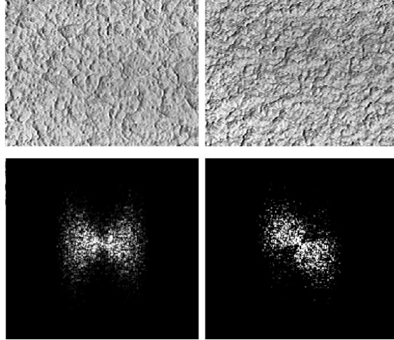
Fig. 13. Changes in the spatial spectrum due to changes in imaging conditions. (Top row) Two images of sample 11 with different illumination and viewing directions. (Bottom row) Spatial spectrum of the images in the top row, with zero frequency at the center and brighter regions corresponding to higher magnitudes. The orientation change in the spectrum is due to the change of illumination direction which causes a change in the shadow direction.
