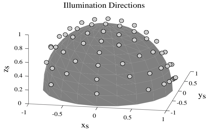
Fig. 5. An alternative interpretation of the measurements described in Figure 4. Illumination directions are shown in the sample coordinate frame. The sample lies in the x_s - y_s plane and its global normal points in the direction of z_s . Each circular marker represents a distinct illumination direction. For each of these illumination directions, the sample is imaged from 7 viewing directions, corresponding to the 7 camera positions shown in Figure 4.
