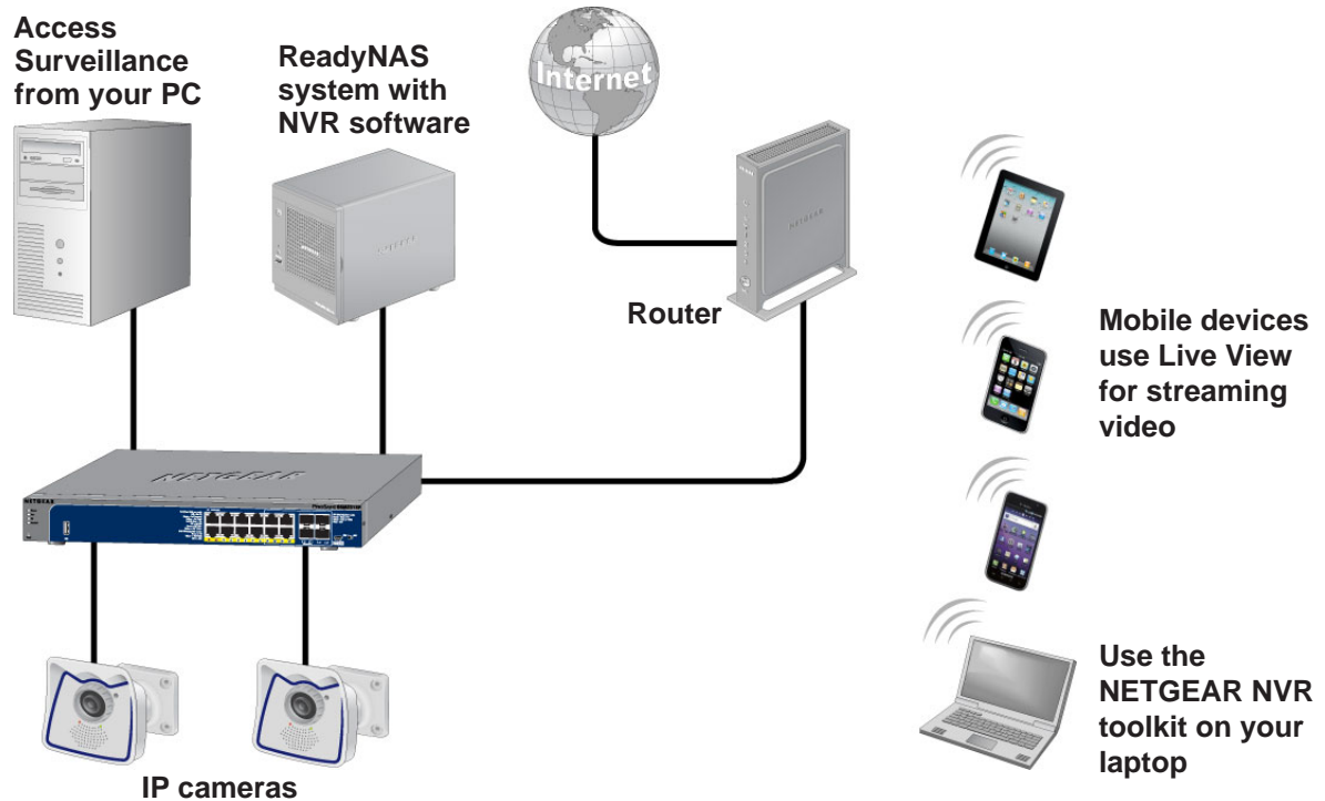
Figure 1. Network with ReadyNAS Surveillance and two IP cameras
