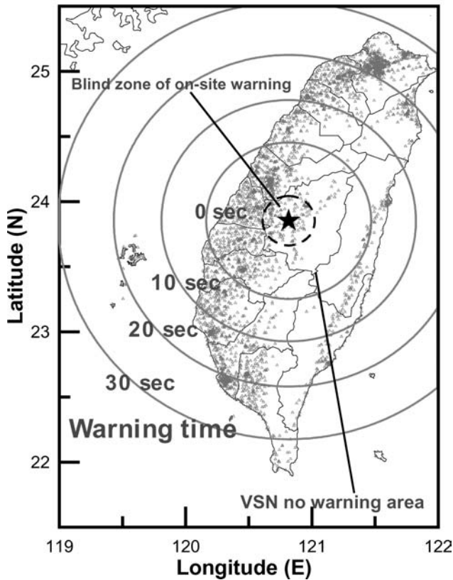
Figure 1 Expected VSN-based EWS early warning times (indicated by solid circles ) in Taiwan with respect to the occurrence of an event similar to the Chi-Chi earthquake of September 20, 1999. Triangles give the location of elementary schools, which can be regarded as the population density of Taiwan. The small circle ( dashed ) with a radius of 21 km indicates the boundary of the blind zone of the on-site warning method.
