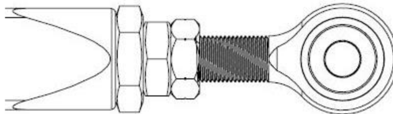
INCORRECTLY ADJUSTED INSUFFICIENT THREAD ENGAGEMENT ON ROD END
